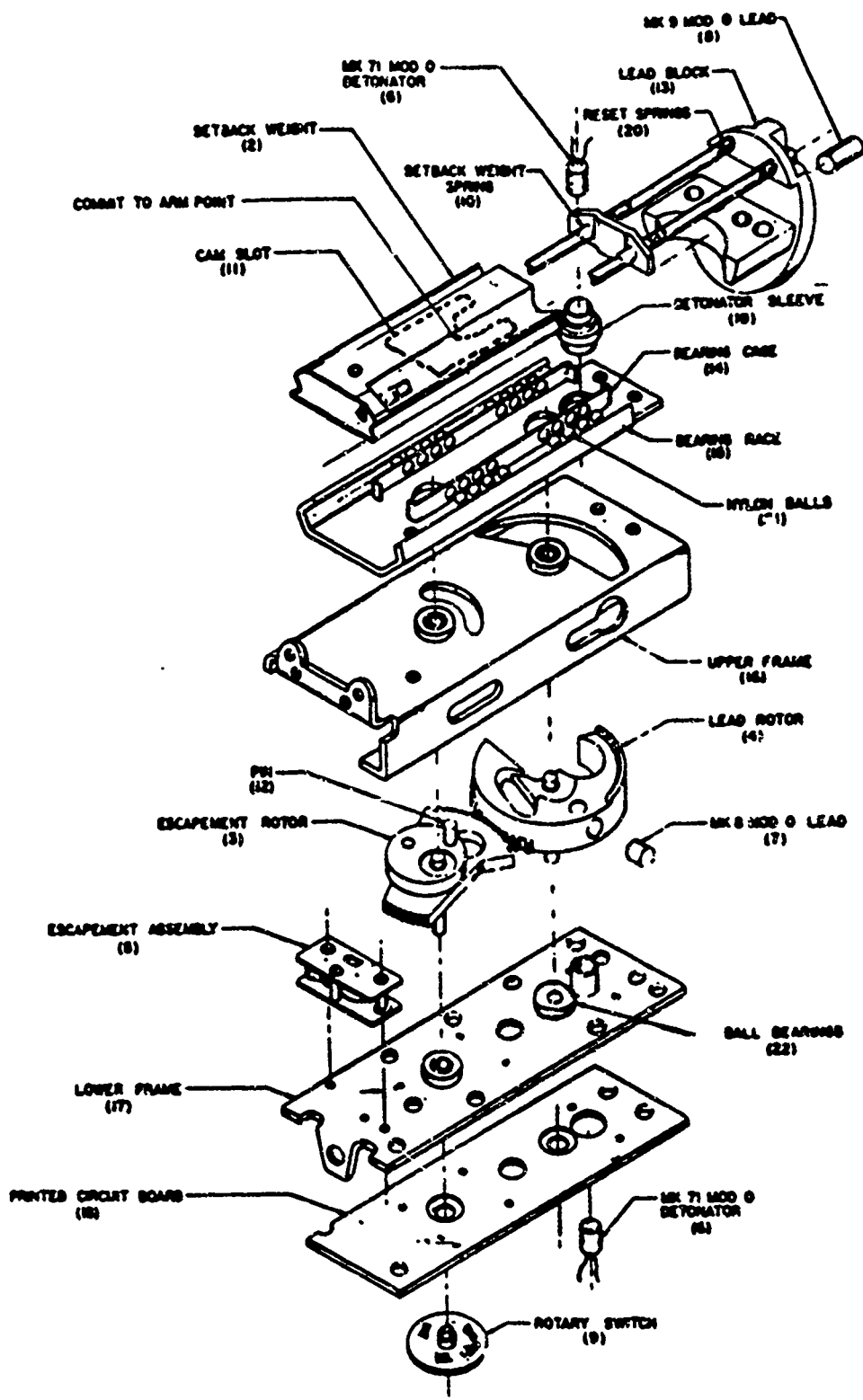
Figure 3. Components of an Electro-Mechanical Fuze
