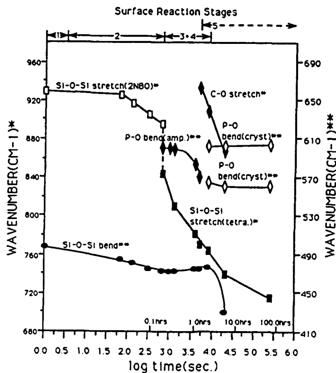
Figure 2: Wavenumber verses time for 45S5(rerun on SXB)
