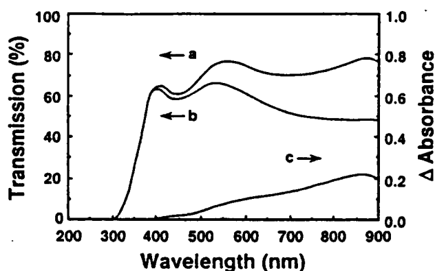
Fig. 2. Optical transmission spectra of a WO 3 -deposited 45BaO-55P 2 O 5 glass and an absorption spectrum of the WO 3 film. Curve a and b are spectra of specimen before and after the dc voltage was applied, respectively. Curve c is the difference spectrum between a and b, which is characteristic of tungsten bronzes.
