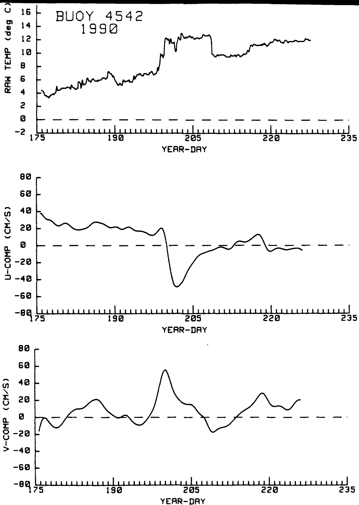
Figure B-5b. Time history of sea surface temperature, U, and V velocity components (filtered) for 4542.
