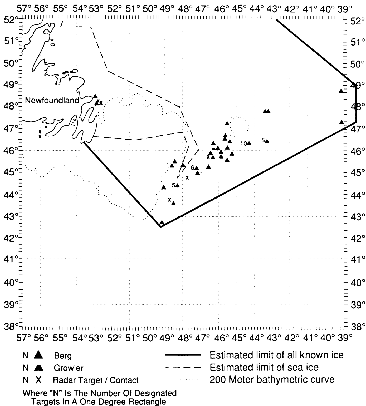
Figure 17. Graphic Depiction Of International Ice Patrol Ice Plot For 1200 GMT 15 Mar 91 Based On Observed And Forecast Conditions
