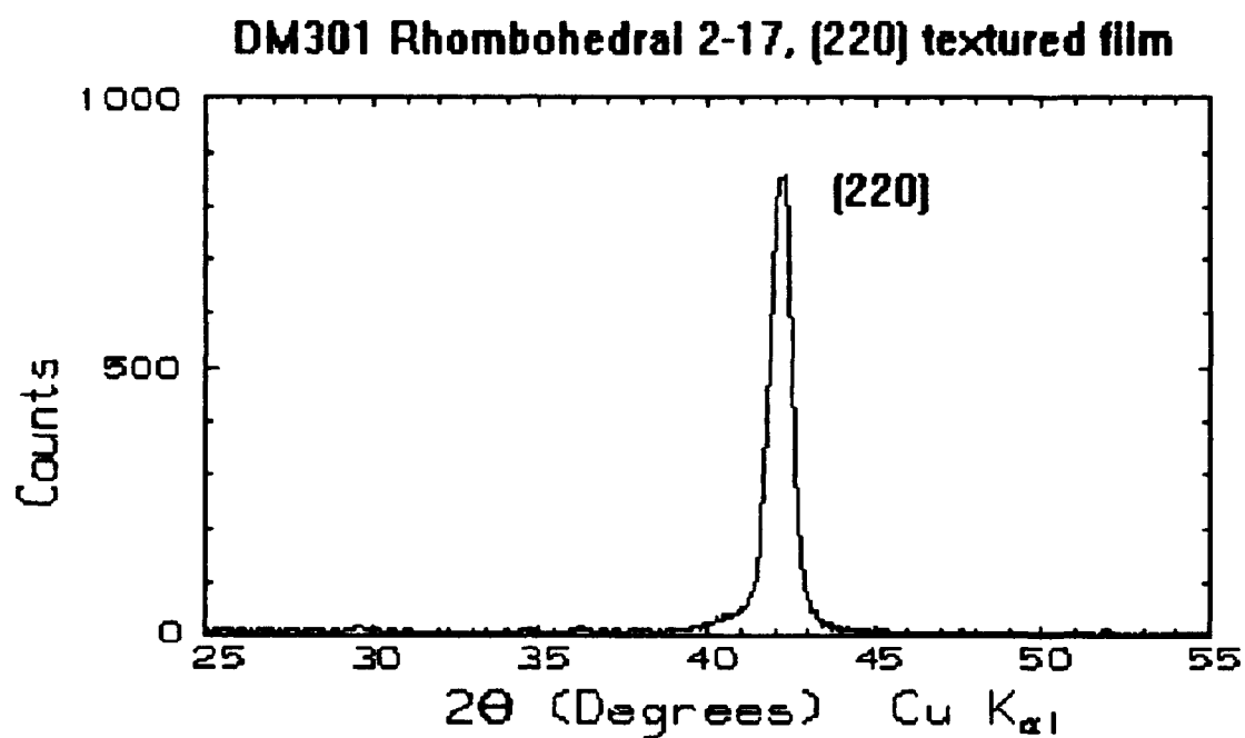
Fig. 7. A \text{CuK}\alpha diffractometer trace for a 2-17 directly crystallized film with (220) texture is shown.
