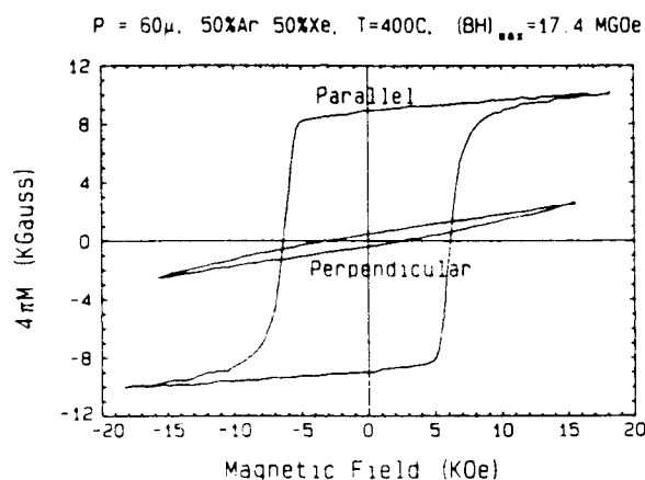
Fig. 2. In-plane and perpendicular to plane hysteresis loops for a 5 \mu\text{m} thick Sm-Co based \text{TbCu}_7 type structure film sputtered with 60 mTorr Ar 50%Xe at a substrate temperature of 400 ^{\circ}\text{C} . These loops were measured at room temperature.
