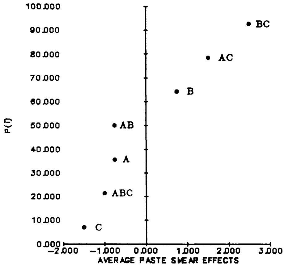
Figure 30. Normal Plot Solder Paste Smear, FPD Parallel Pads
