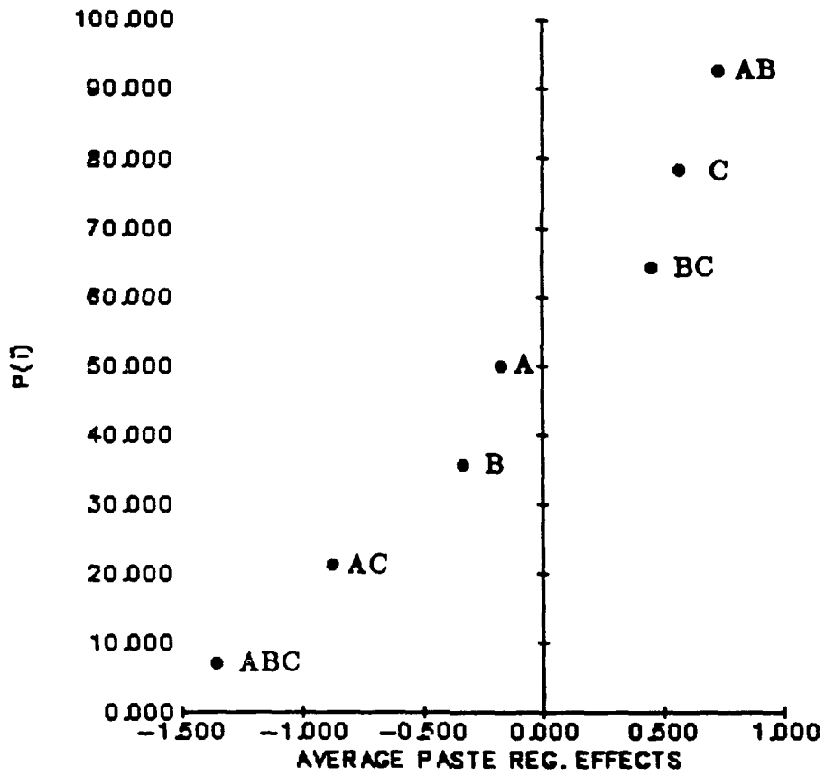
Figure 29. Normal Plot Solder Paste Registration, Lower Right Corner
