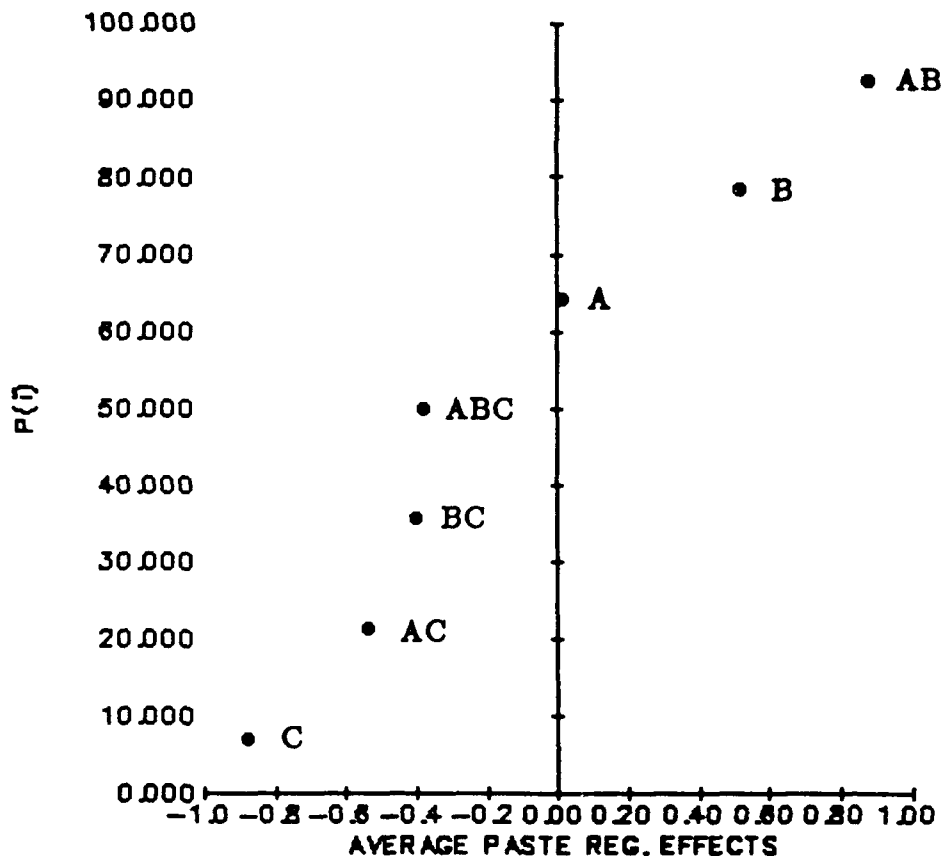
Figure 27. Normal Plot Solder Paste Registration, Upper Right Corner
