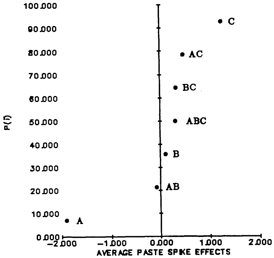
Figure 38. Normal Plot Solder Paste Spikes, FPD Parallel Pads
