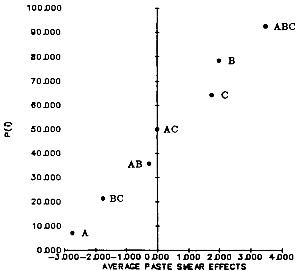
Figure 32. Normal Plot Solder Paste Smear, LCC Parallel Pads
