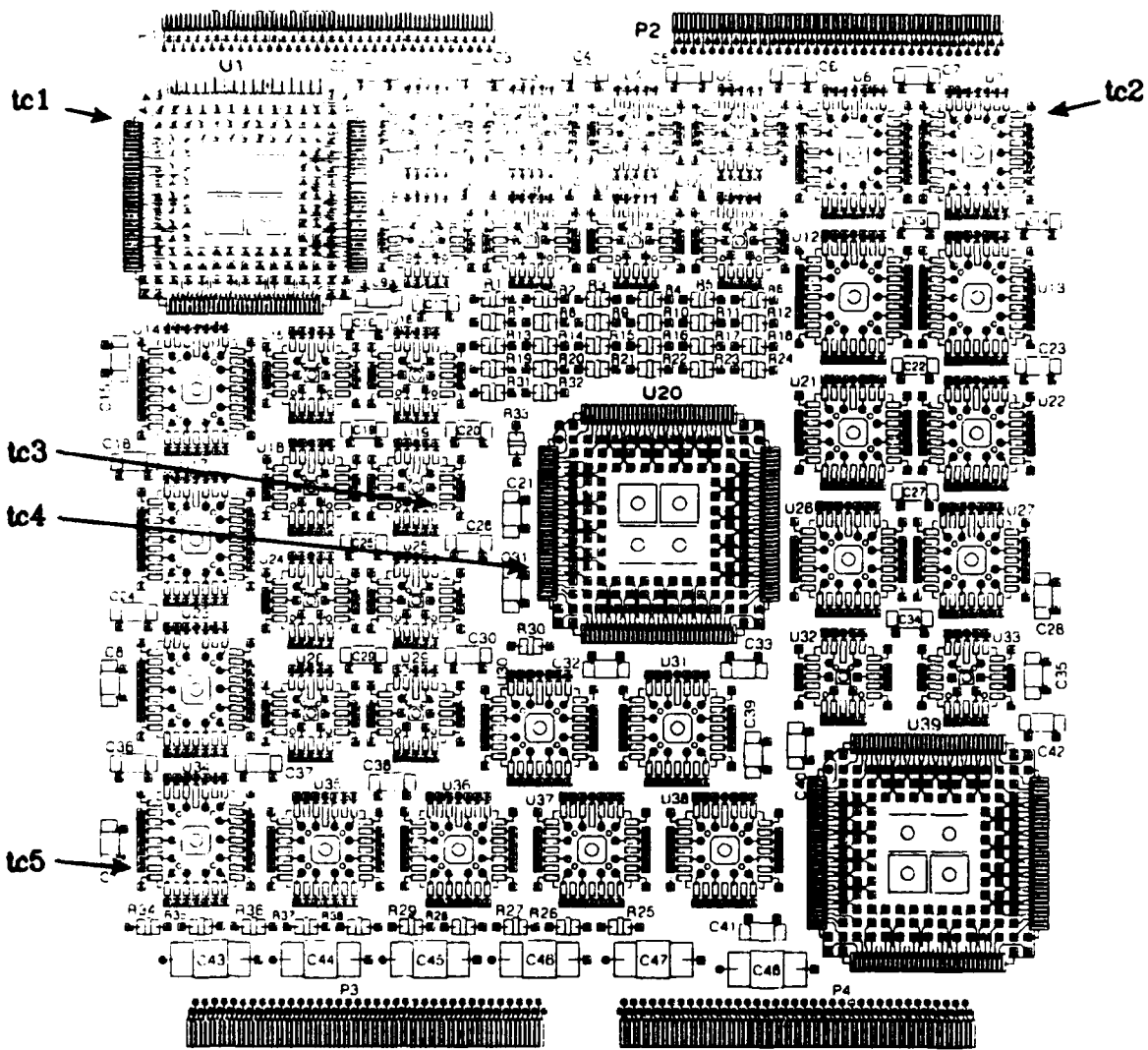
Figure 9. EMPI PWB Showing Thermocouple Bead Locations
