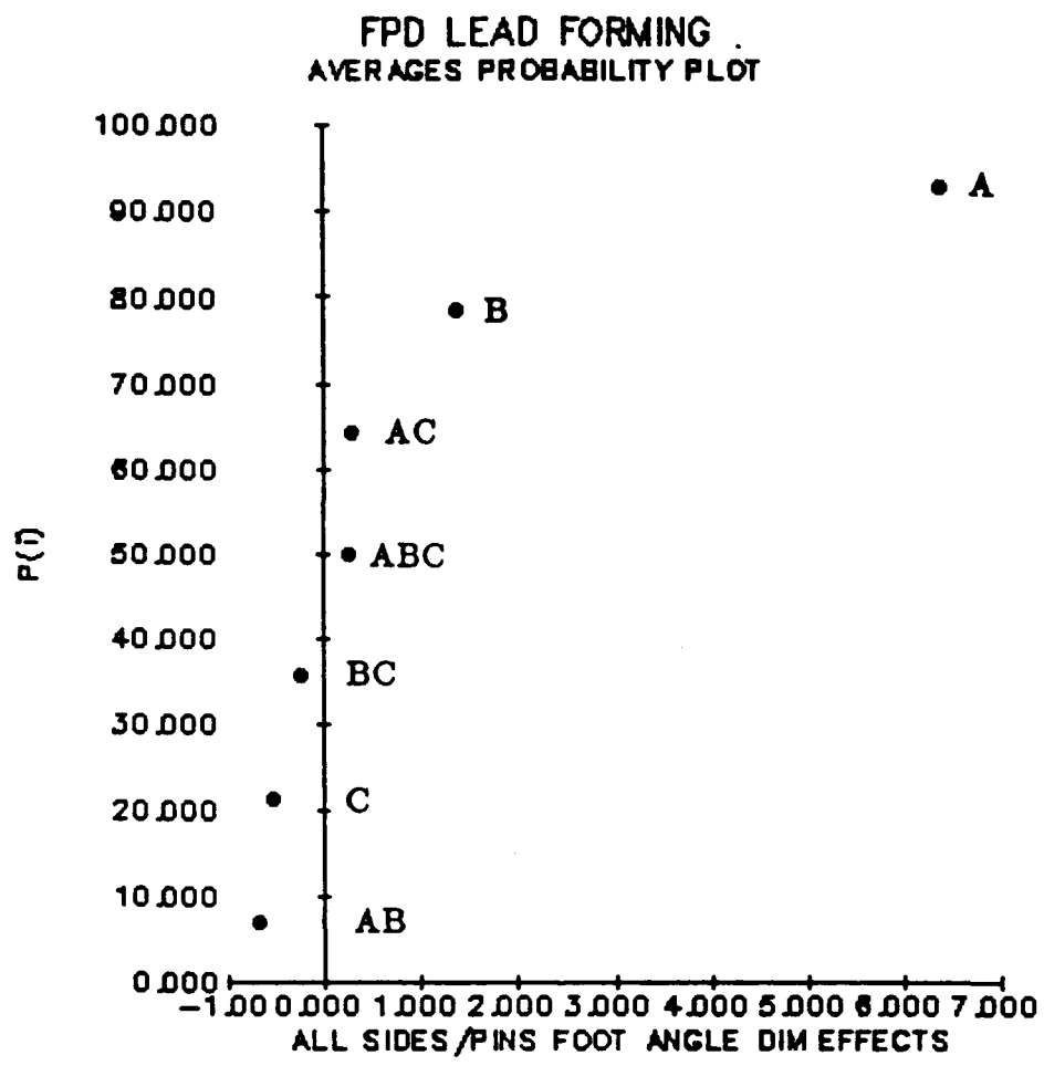
Figure 23. Normal Plot FPD Toe Angle Dimension
