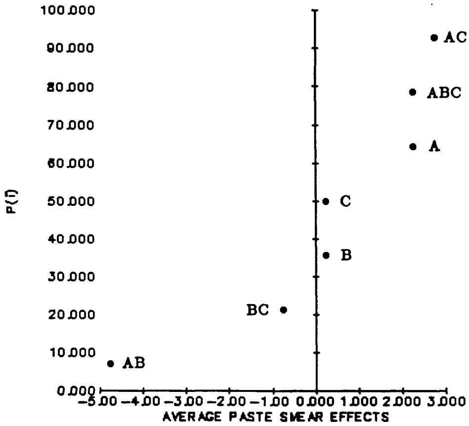
Figure 33. Normal Plot Solder Paste Smear, LCC Perpendicular Pads
