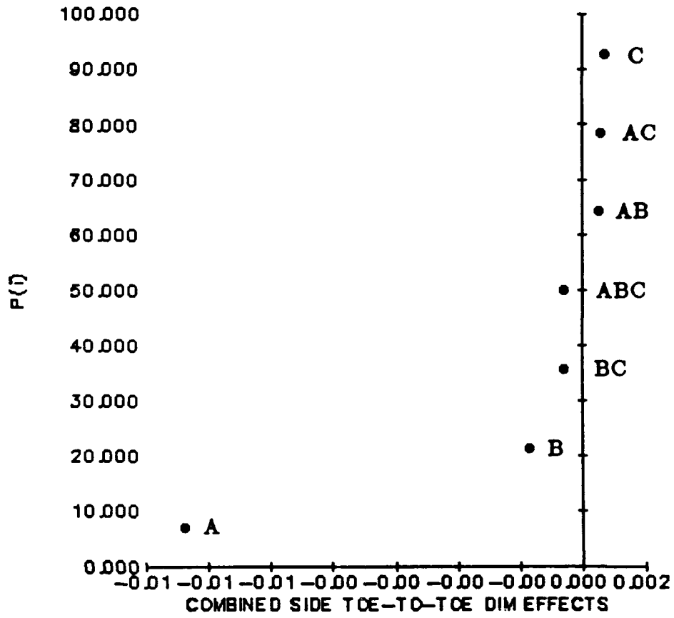
Figure 22. Normal Plot FPD Lead Toe-to-Toe Dimension
