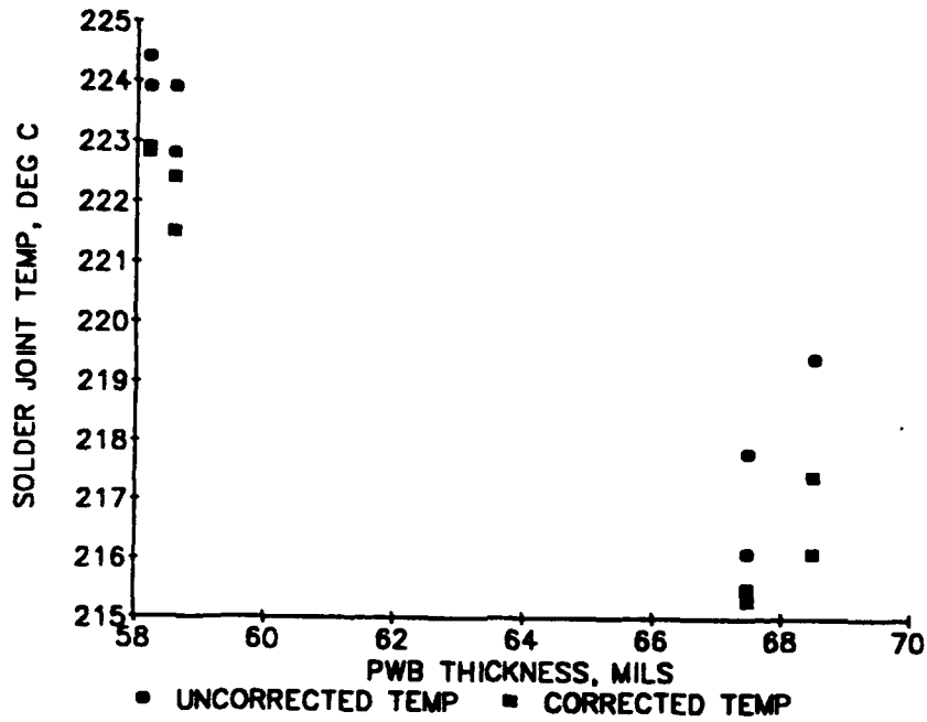
Figure 10. Plot of PWB Thickness Versus Corrected and Uncorrected Solder Joint Temperatures
