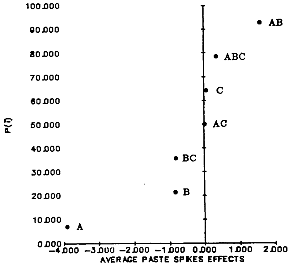
Figure 39. Normal Plot Solder Paste Spikes, FPD Perpendicular Pads
