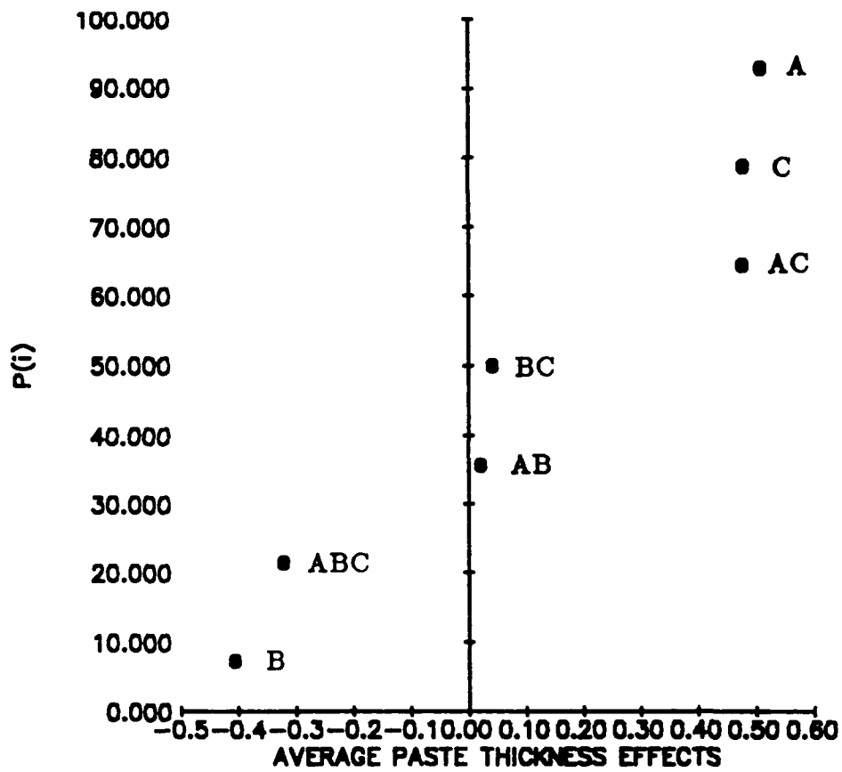
Figure 36. Normal Plot Solder Paste Thickness, LCC Parallel Pads
