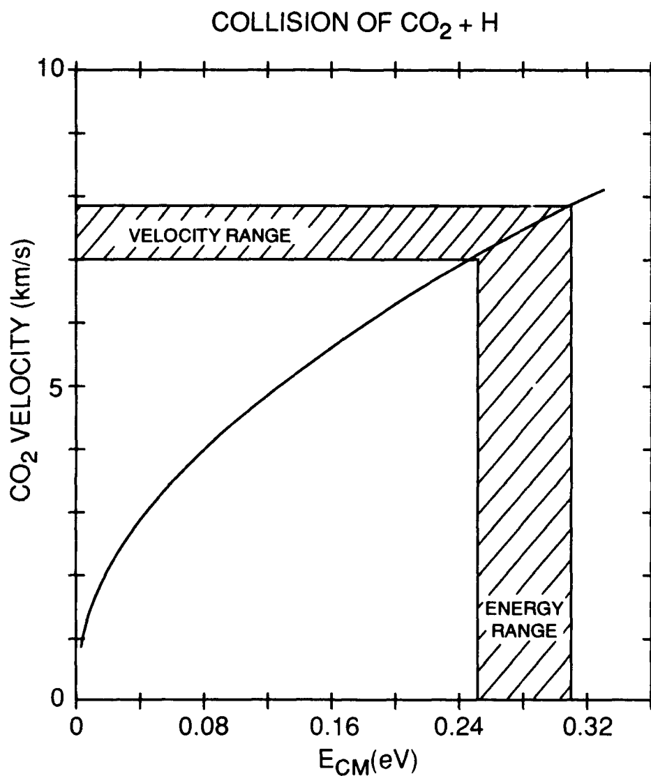
Figure 14. The Center of Mass Energy Range, Bracketed by the Forward and Backward Release Cases, for the Collision \text{CO}_2 + \text{H}
