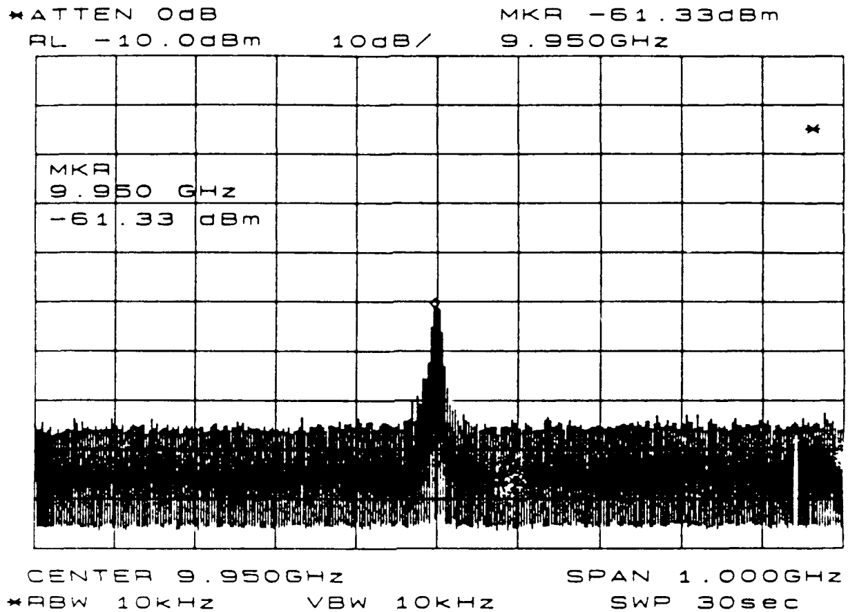
Fig. 5.7 Typical RIN noise spectrum of the external cavity laser.
