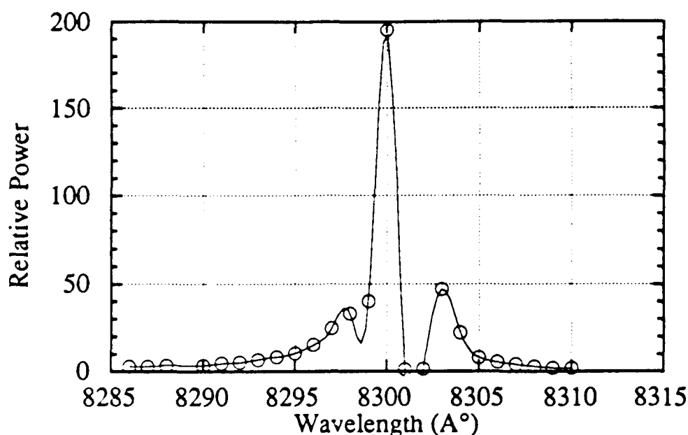
Fig. 5.14 The lasing spectrum.
