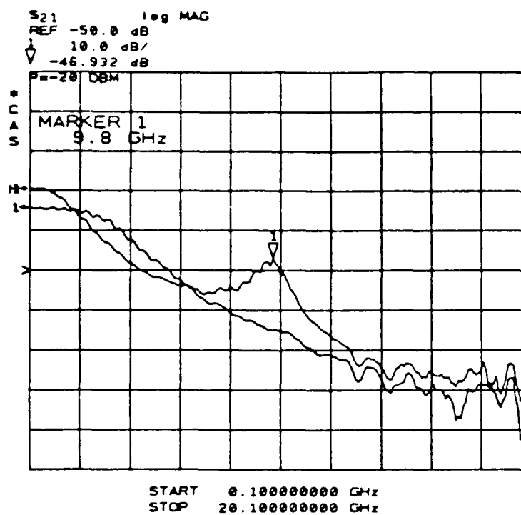
Fig. 5.17 Experimental laser response for 10 GHz cavity at -20 dBm.
