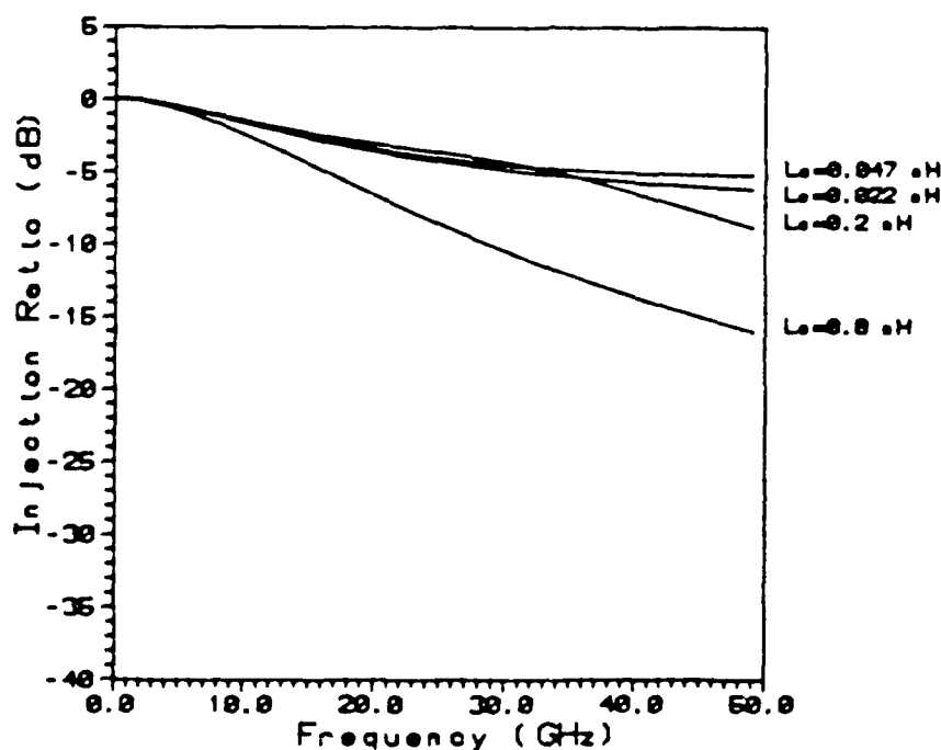
Fig. 4.6 Current injection for R_L=9 \Omega , Z_g=50 \Omega , C_p=2 \text{ pF} , & C_T=0.1 \text{ pF} .
