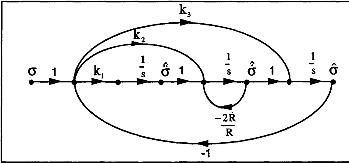
Figure 10. Luenberger Observer for estimating \dot{\sigma} and \ddot{\sigma}
