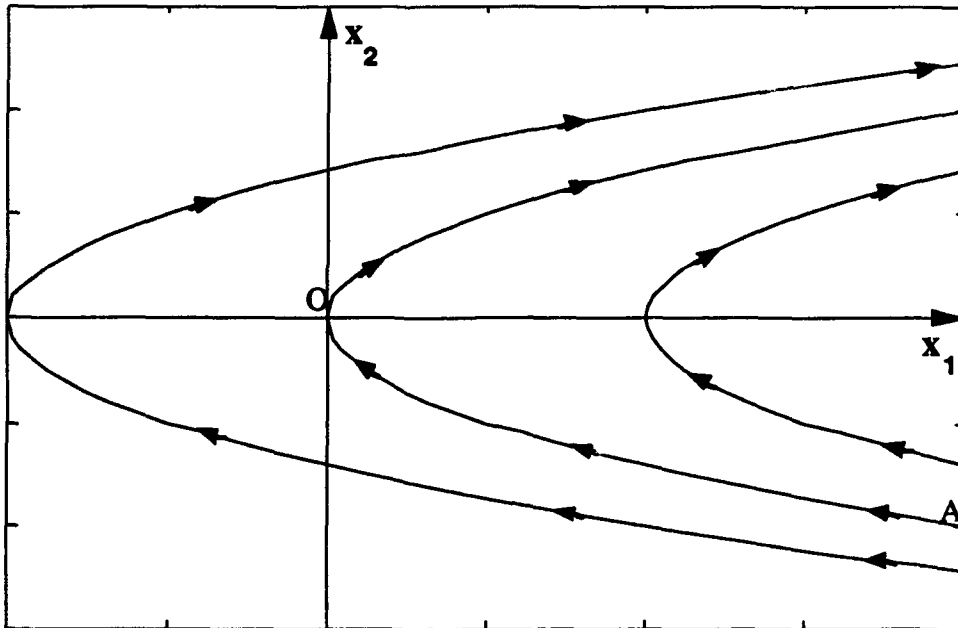
Figure 3. Trajectories for u=+N
