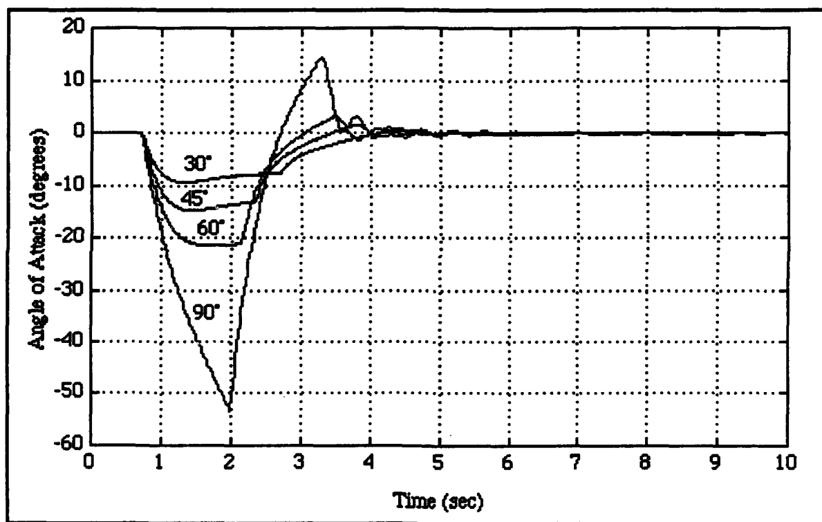
Figure 18. Missile Boost Phase Angle of Attack Profiles
