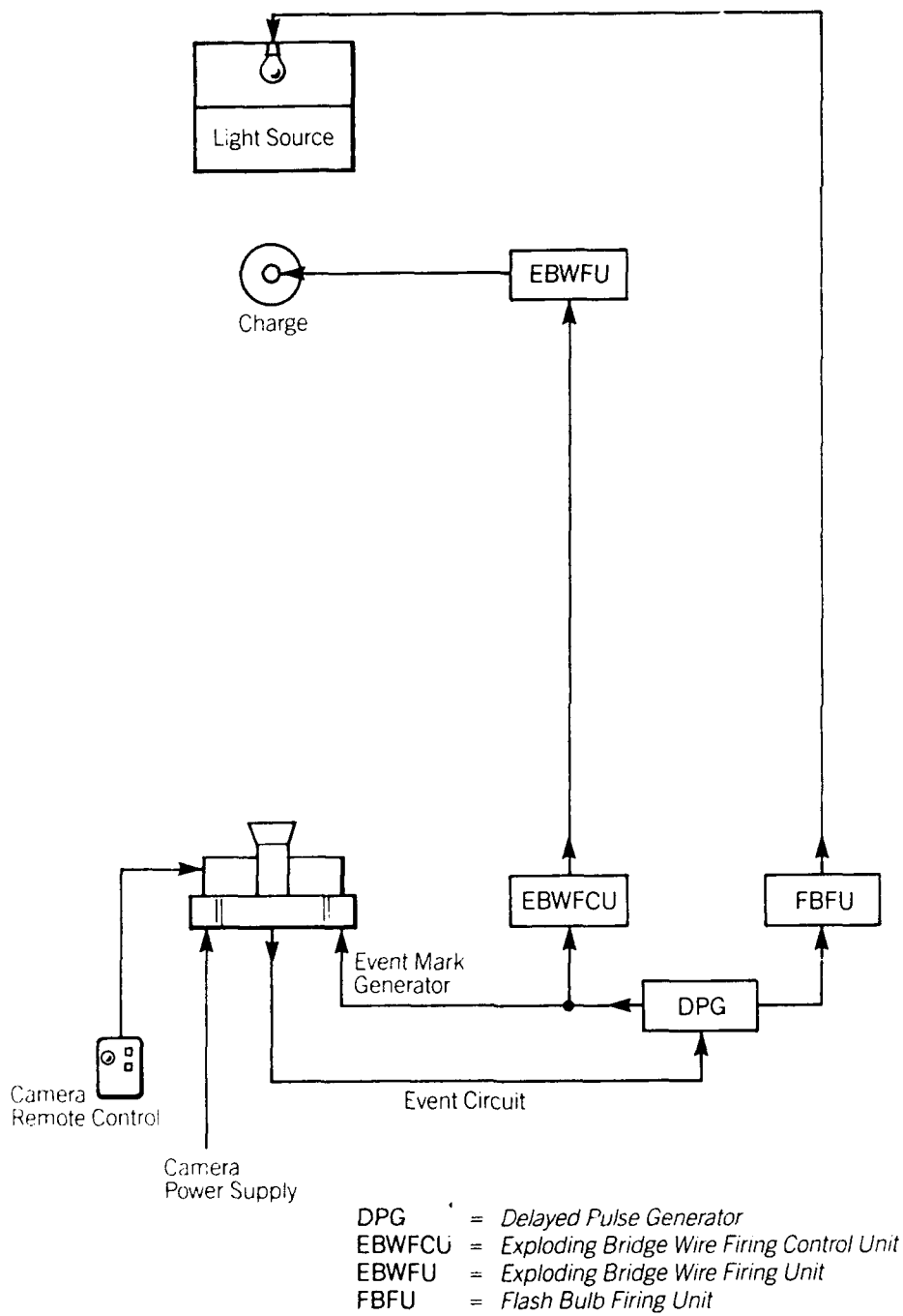
Figure 3: Instrument schematic diagram.
