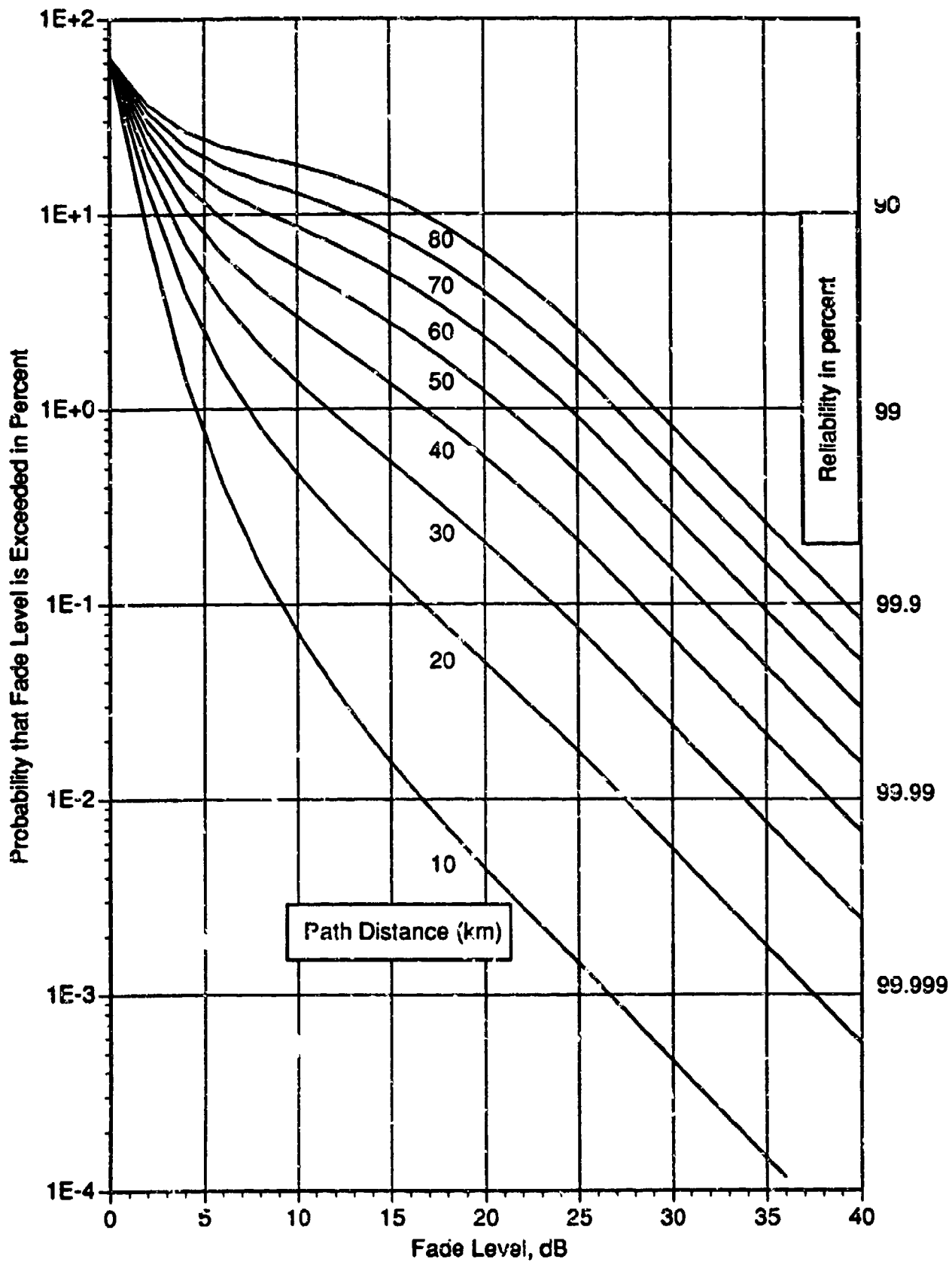
Figure A-5A. Probability of Fading (1600 MHz, Difficult Climate)
