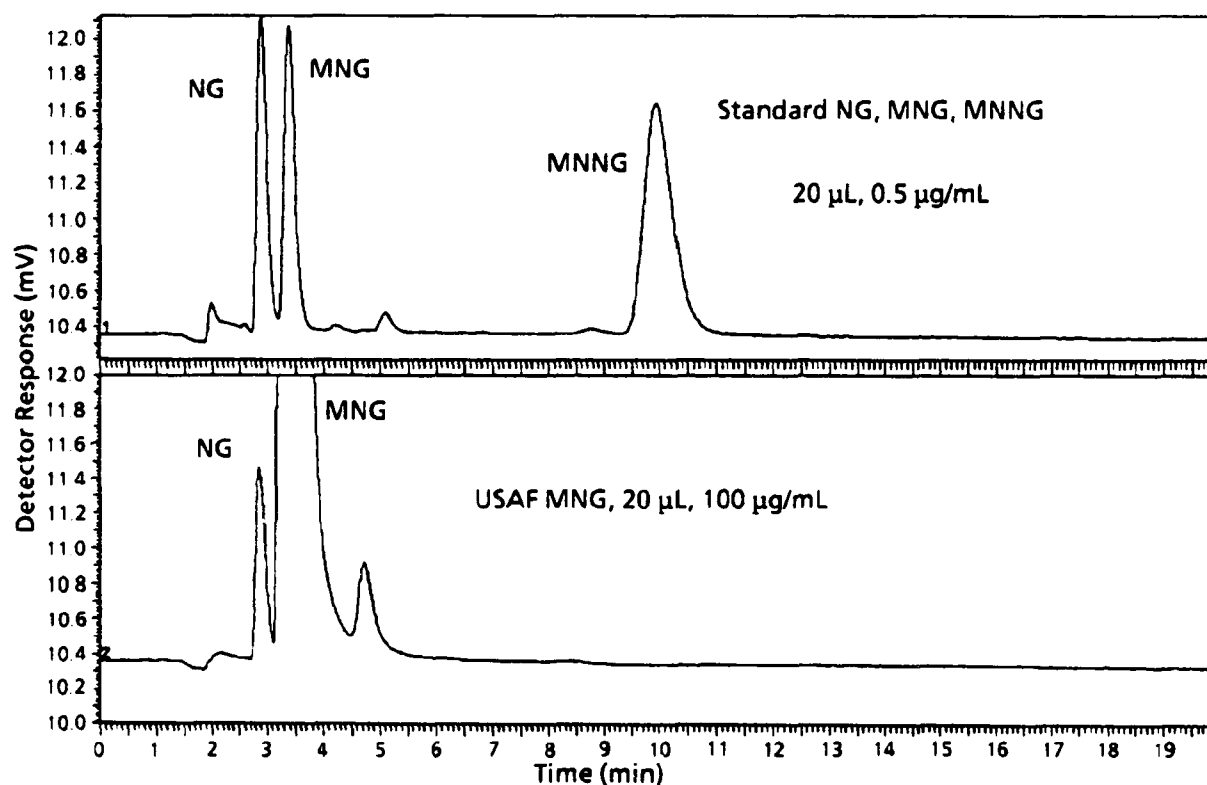
Figure 4. Analysis of Air Force Armament Laboratory MNG by HPLC with UV Detection. Top panel: Aqueous standards of 0.5 µg/mL NG, MNG, and MNNG. Bottom panel: Expanded chromatogram showing small amount of NG in Air Force MNG.
