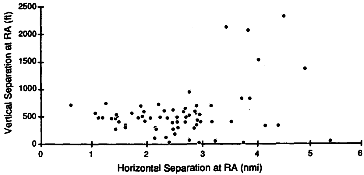
Figure 18. Separation at Approximate Time of Corrective RAs at Dallas-Ft. Worth
