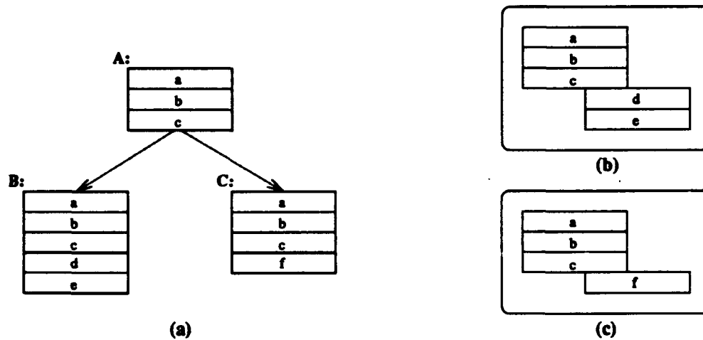
Figure 9: Subclassing as a Specialization Evolution: The standard subclassing mechanism could be implemented using a restricted form of class versioning and instance adaptation. Figure (a) depicts three classes: B and C as subclasses of A. Figure (b) presents Class B as a new version of A. Figure (c) does likewise for C. Like the formal subclasses, the versions depicted in (b) and (c) can substitute for (i.e., are compatible with) instances of A.
