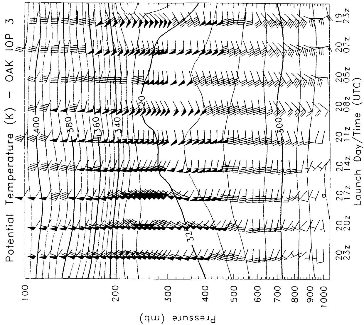
Fig. 11 As in Fig. 3, except for Oakland (OAK).
