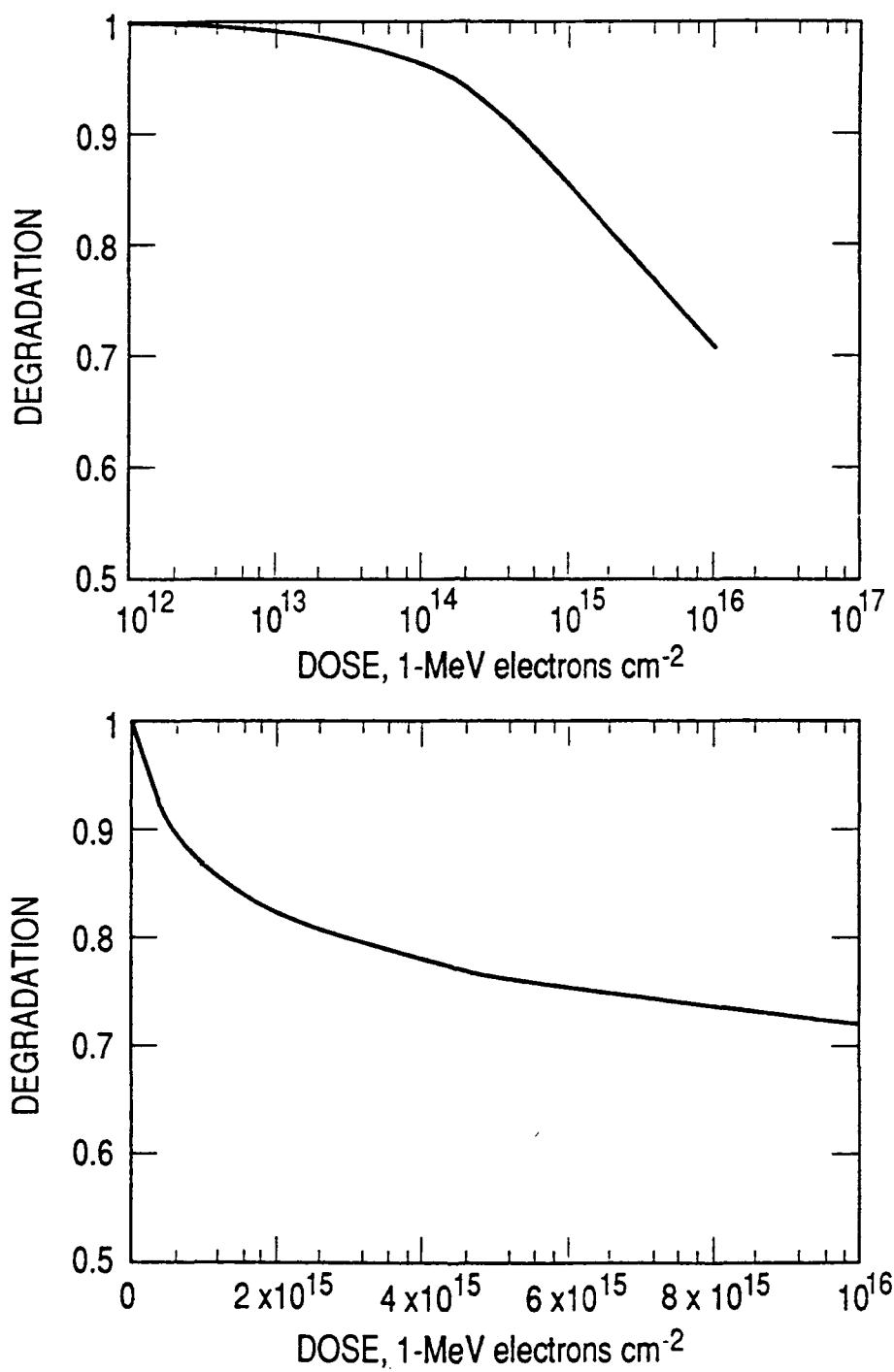
Fig. 6. Normalized I_{sc} vs 1-MeV electron fluence for 10 ohm-cm n/p, BSR silicon cells. Linear and semilogarithmic plots contain the same data.
