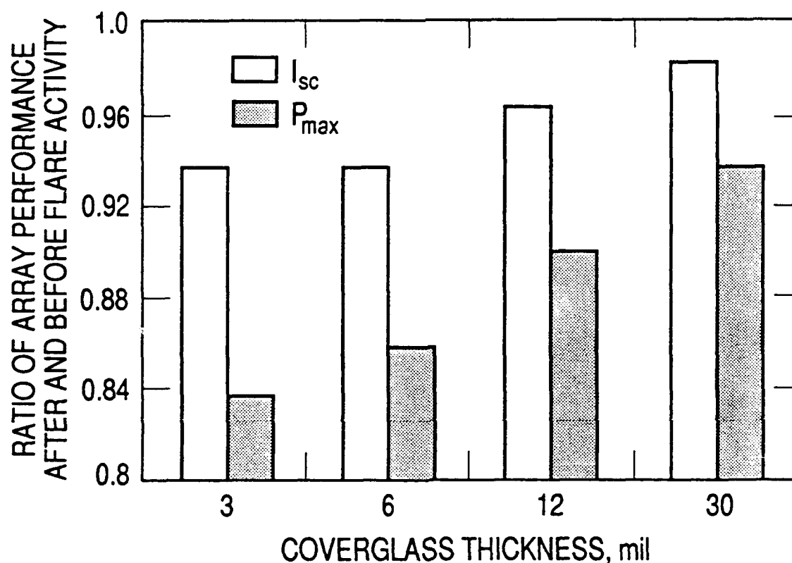
Fig. 8. Calculated effects of 20 October 1989 flare on a K7 solar cell.
