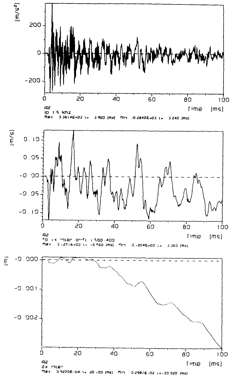
Figure 30 Accelerometer A2
