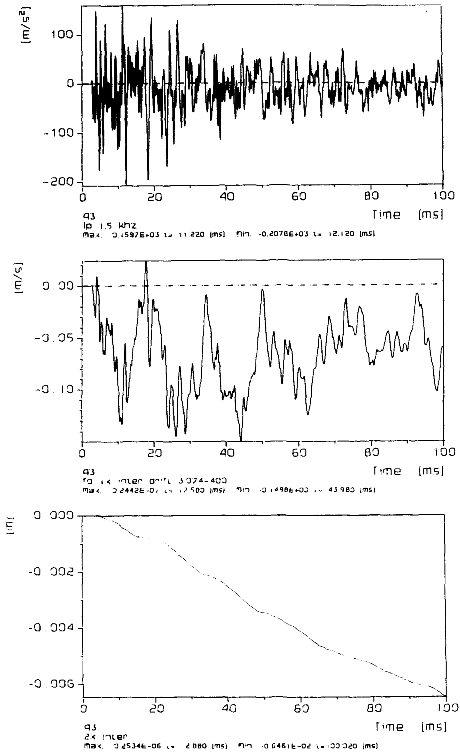
Figure 31 Accelerometer A3
