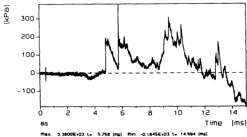
Figure 6 Pressure signals B3, B4 and B5 (BHD 78)
