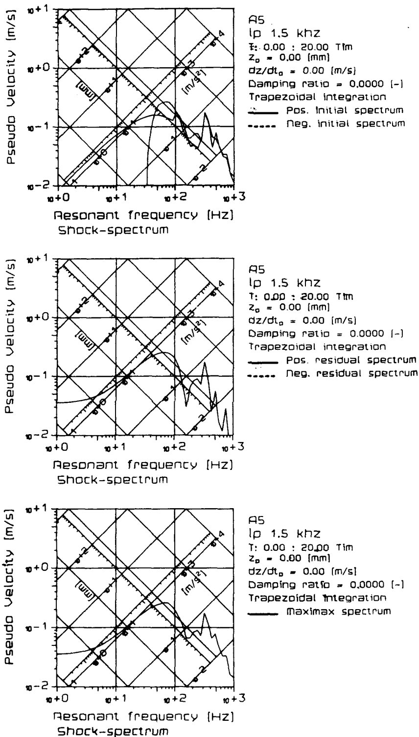
Figure 40 Shock spectra accelerometer A5
