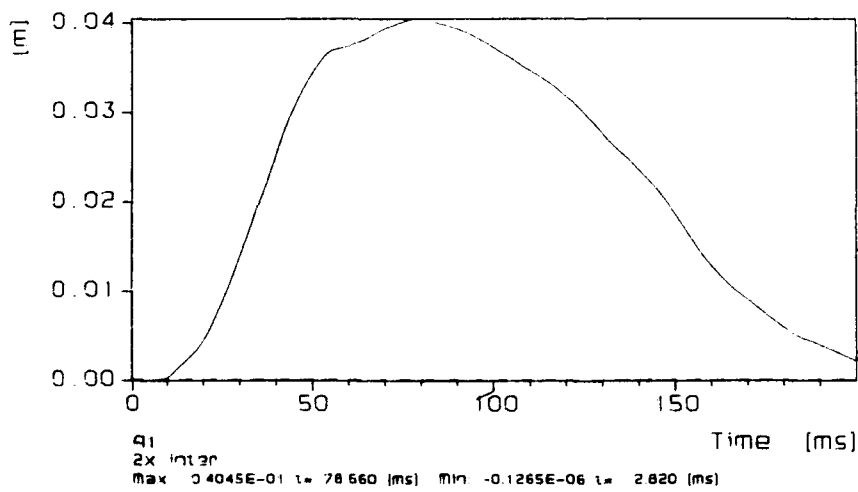
Figure 29 Accelerometer A1
