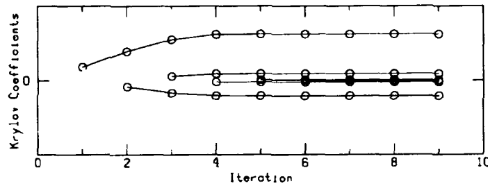
Figure 15 - Iteration history of coefficients for Poisson equation example.
