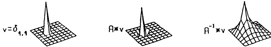
Figure 3 - The sparsity of A (discrete Poisson operator) and A^{-1} (discrete Green's function) contrasted by their action on a sample \delta -function on a two-dimensional grid.
