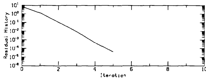
Figure 17 - Iteration history for ILU-preconditioned Poisson equation example, Euclidean norm of residual.
