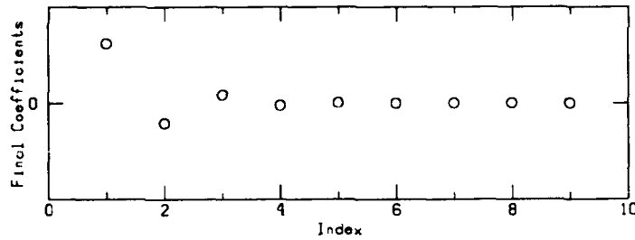
Figure 14 - Converged coefficients of the Krylov vectors of Fig. in the solution of Fig. .
