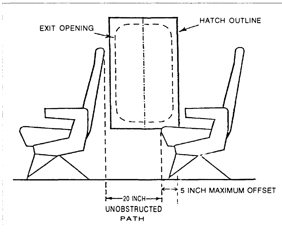
FIGURE 1. CONFIGURATION "A"
