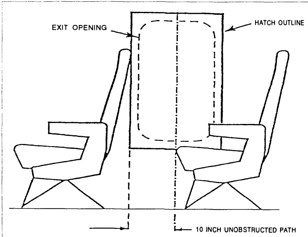
FIGURE 3. CONFIGURATION "C"
