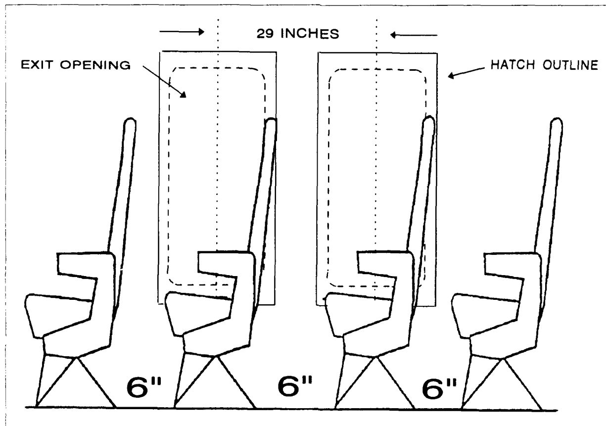
FIGURE 4. CONFIGURATION "D"
