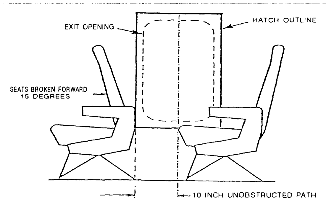
FIGURE 2. CONFIGURATION "B"
