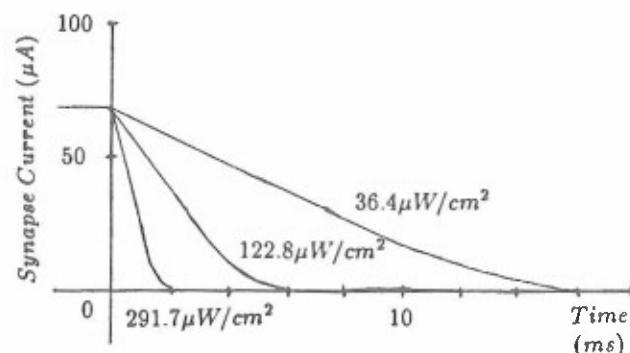
Fig. 20. Synaptic time response dependence on light intensity.
