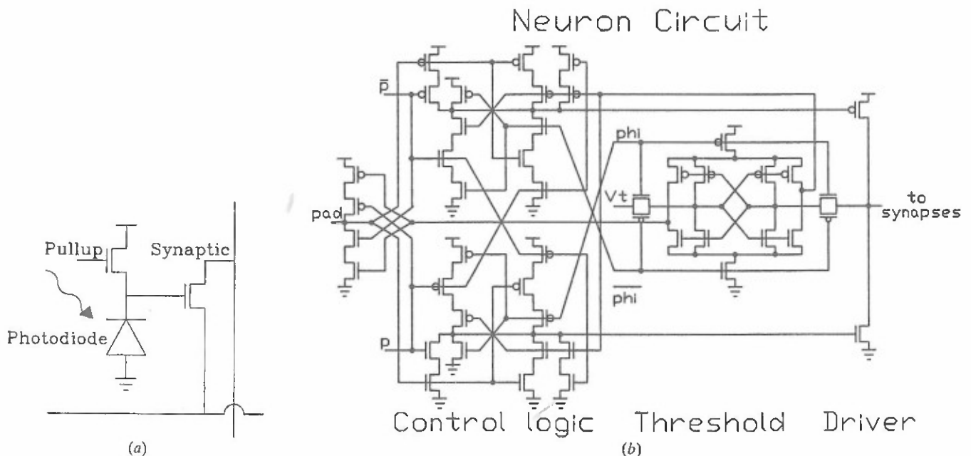
Figure 9. Circuit diagrams: (a) synapse, (b) neuron.
