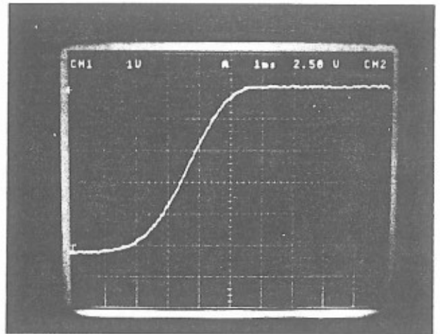
Figure 10. Synaptic current ( 6.67 \mu\text{A} per vertical division) versus optical illumination time ( 1 \text{ ms} per horizontal division).
