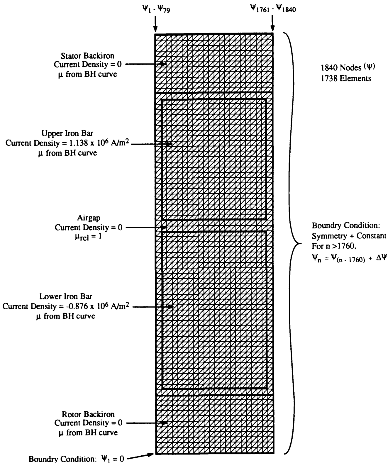
Fig. 17. Finite Element Model Showing the Elements Used and Boundary Conditions for the Case Where the Armature Current is 35 kA. The Corner of Each Triangular Element Represents a Node, Numbered 1 to 1840 Starting From the Lower left Hand Corner.
