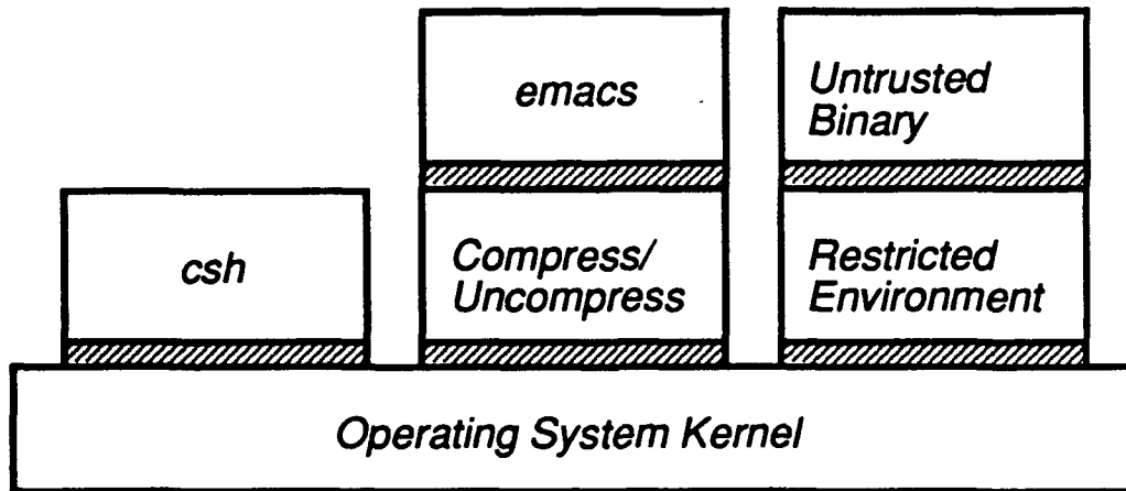
Figure 1-3: Kernel and agents provide instances of system interface
