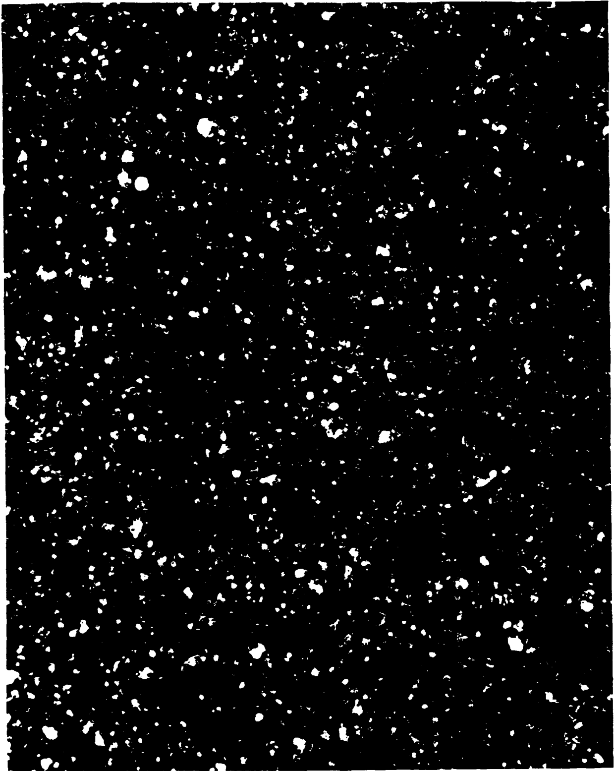
Fig. 3. Nanograin spinel of composition MgO.1.25Al_2O_3 , having an average grain size of 38 nm. The material was codeposited with 1.3 vol % Pt by PVD in an amorphous form and then annealed at 1100°C to produce the nanocrystalline structure.
