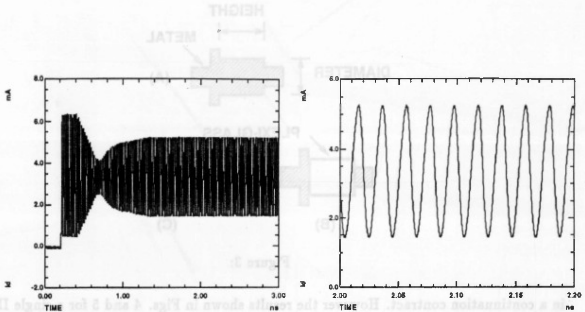
Figure 4: Current through IMPATT diode.
