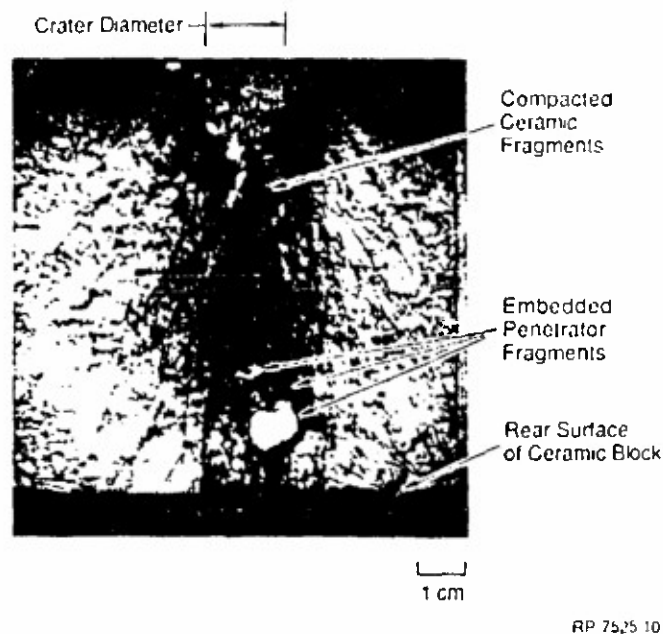
FIG. 5. Cross-section through shot line of 100 mm thick confined B_4C target impacted at a higher velocity showing cracking pattern, compacted ceramic fragments in cavity produced by penetrator and embedded penetrator fragments.
