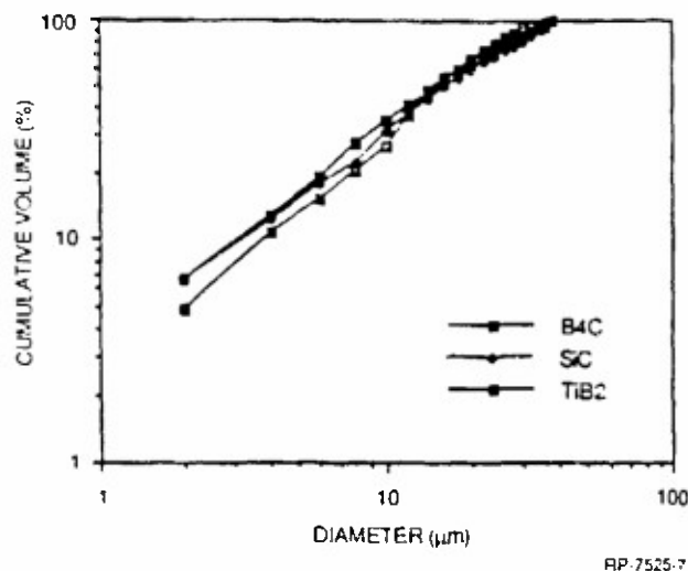
FIG. 4. Distribution of fragments of B_4C , SiC and TiB_2 in the 2–40 \mu m size range.
