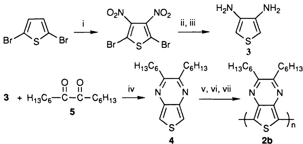
Scheme 1 Reagents and Conditions: i, fuming \text{HNO}_3 , fuming \text{H}_2\text{SO}_4 , 20–30 °C; ii, Sn, HCl, 30 °C then 0 °C; iii, 4N NaOH/ ether; iv, ether/MeOH, reflux, followed by TLC; v, \text{FeCl}_3 , \text{CHCl}_3 , dry air, 50 °C, 3 d; vi, \text{N}_2\text{H}_4/\text{H}_2\text{O} ; vii, dialysis in \text{CHCl}_3 (MW cutoff 3,500) and precipitation with MeOH.
