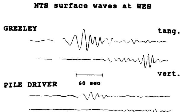
Fig. 1. Love and Rayleigh waves from two nuclear explosions with high levels of tectonic release (PILE DRIVER and GREELEY) recorded at WES (a WWSSN long-period seismic station). The vertical and tangential components are on the same scale. From Toksöz and Kehrler [1972].
