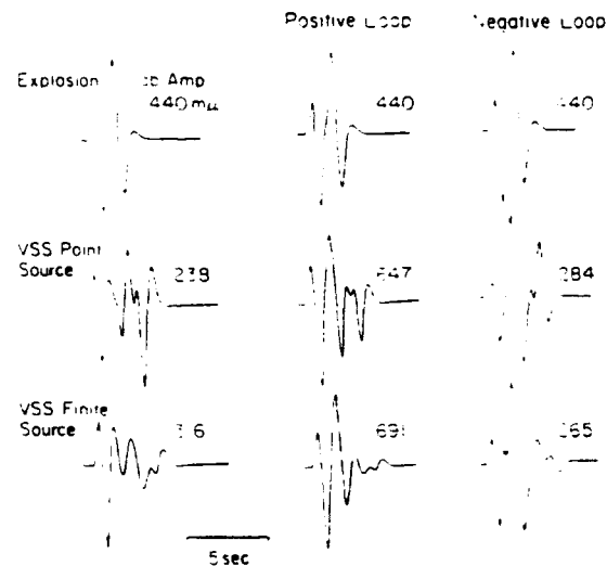
Fig. 9. A simulation of the short-period P waveforms for GREELEY assuming a vertical strike-slip (vss) orientation for the tectonic release. Top trace is the explosion alone. Next row is the effects of a point source tectonic release (left column is tectonic release alone, middle column is explosion plus tectonic release in the positive P loop direction, and the right column is the sum of the explosion and tectonic release in the negative P loop direction), and downward rupturing P wave synthetic. From Lay et al. (1984).
