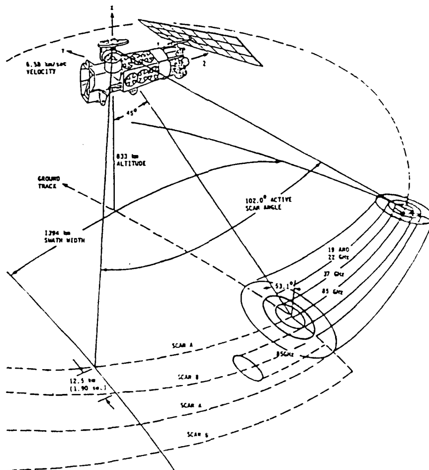
FIGURE 3.0-3 ACTIVE SCAN GEOMETRY
