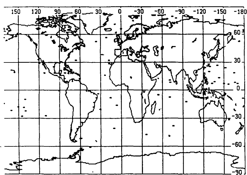
Radiosonde Locations used for SSM/I-TPW Quality Control.
