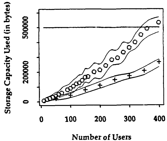
Figure 5: Average quantity of SCU storage used. Circles correspond to 2000 byte maximum message length, while pluses show the results for 1000 byte messages. The surrounding curves show the 95% confidence interval widths for each point. The horizontal line shows the current storage maximum of 500 kilo-bytes in the SCU.
