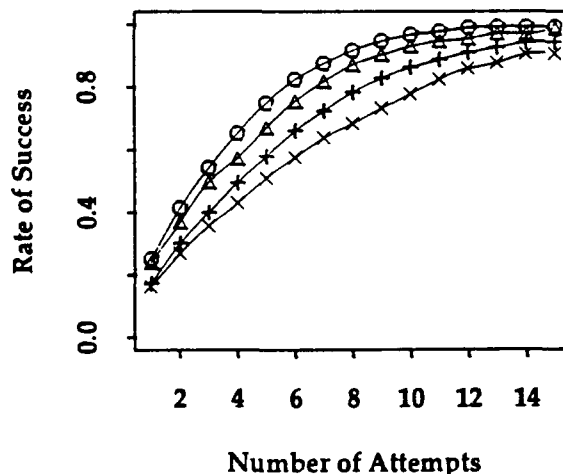
Figure 7: Proportion of user attempts resulting in successful access of the SCU. The circles represent data points for 2400 BPS for bit error probabilities of 10^{-6} and 3 \times 10^{-6} . The plusses and crosses are for 1200 BPS, bit error probabilities of 10^{-6} and 3 \times 10^{-6} .
