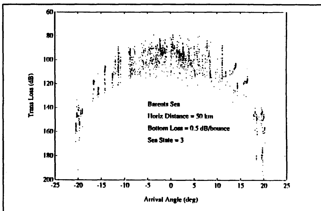
Figure 25 Individual ray transmission loss versus arrival angle for a near bottom sound source (A) at a sea state of 3.
