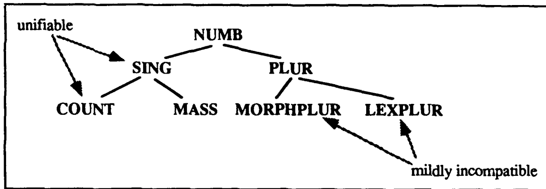
Figure 5: Elastic unification in type hierarchies of features
