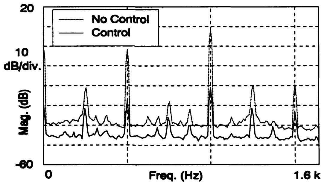
Figure 6.14 Intensity Signal, Short Error Intensity Control, Moment Actuator, 488 Hz, Setup 2.
