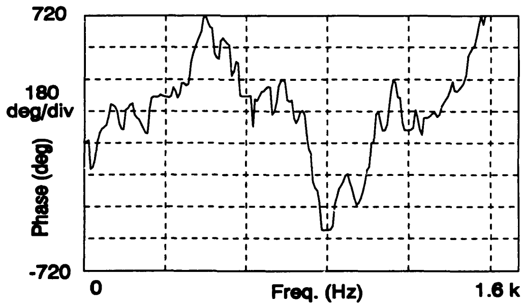
Figure 6.4 Phase of Input Intensity at 300 Hz.
