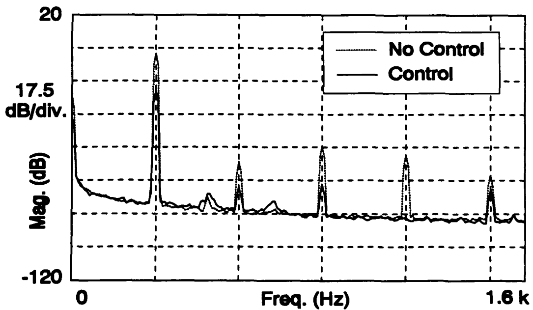
Figure 6.8 Downstream Acceleration, Acceleration Control, 296 Hz, Setup 4.
