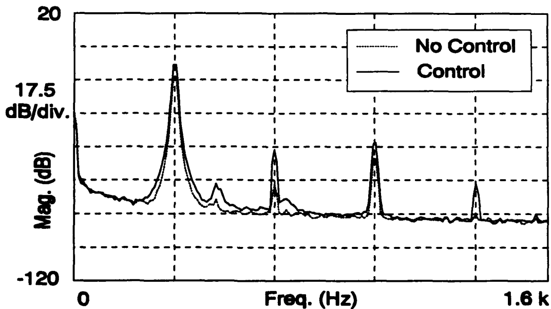
Figure 6.22 Downstream Acceleration, Short Error Intensity Control, Force Actuator, 340 Hz, Setup 4.
