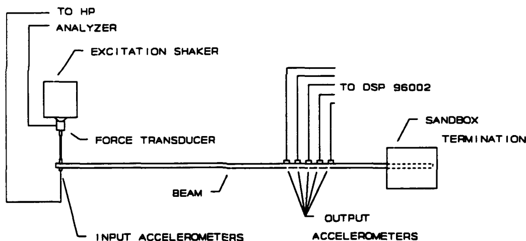
Figure 5.2 Experimental Setup for Intensity Measurement.
