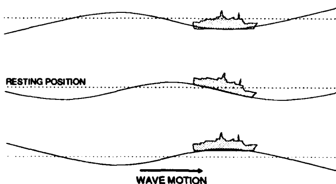
FIGURE 20. EXAMPLE OF ORDINARY WAVE MOTION
