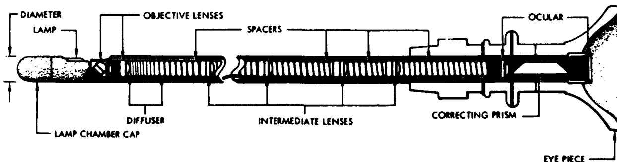
FIGURE 1. TYPICAL BORESCOPE CONSTRUCTION
