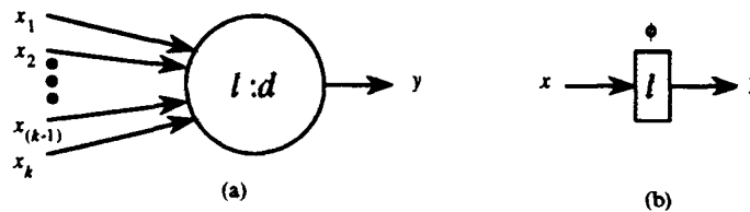
Figure 3: (a) A functional element has some finite number k of inputs x_1 through x_k , a single output y , an associated k -input function f , and a propagation delay d . (b) A level-clocked latch has a single input x , a single output y , and an associated digital clock \phi .
