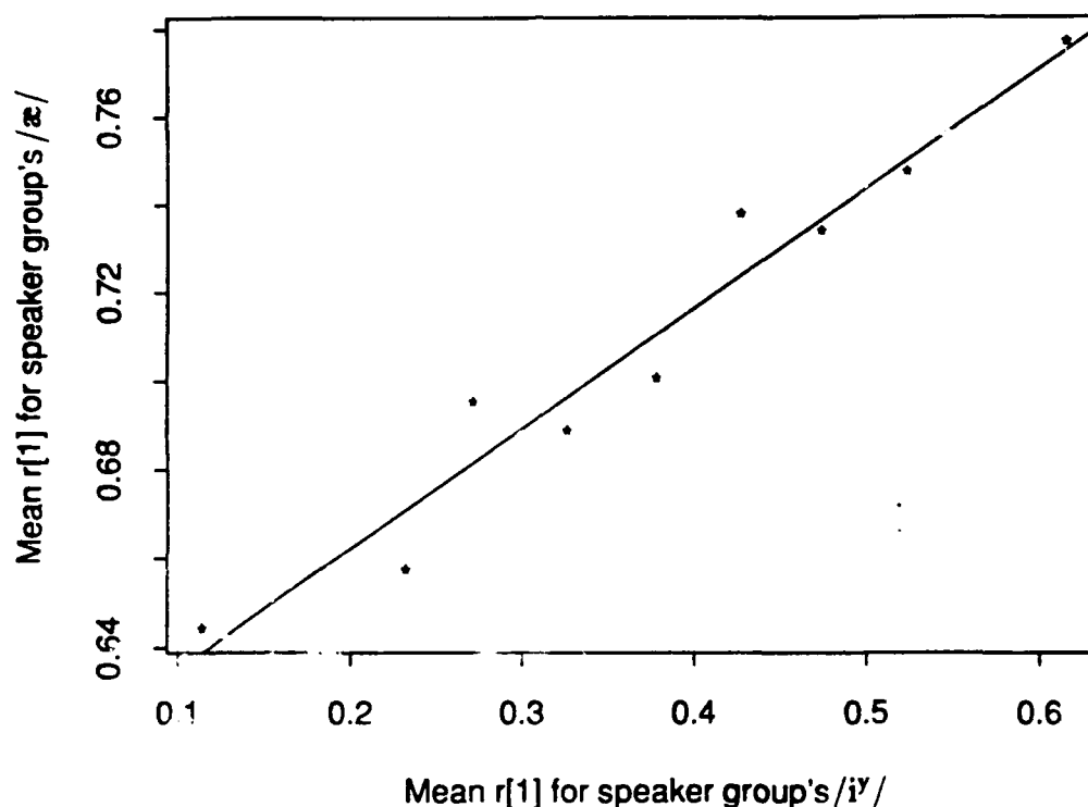
Figure 2.2: Plot of average r[1] values for /iʏ/'s and /æ/'s of each speaker group. Each point represents a speaker group. The x-coordinate of the point is the mean r[1] for /iʏ/'s of all speakers in the group. The y-coordinate is the mean r[1] for the group's /æ/'s.
