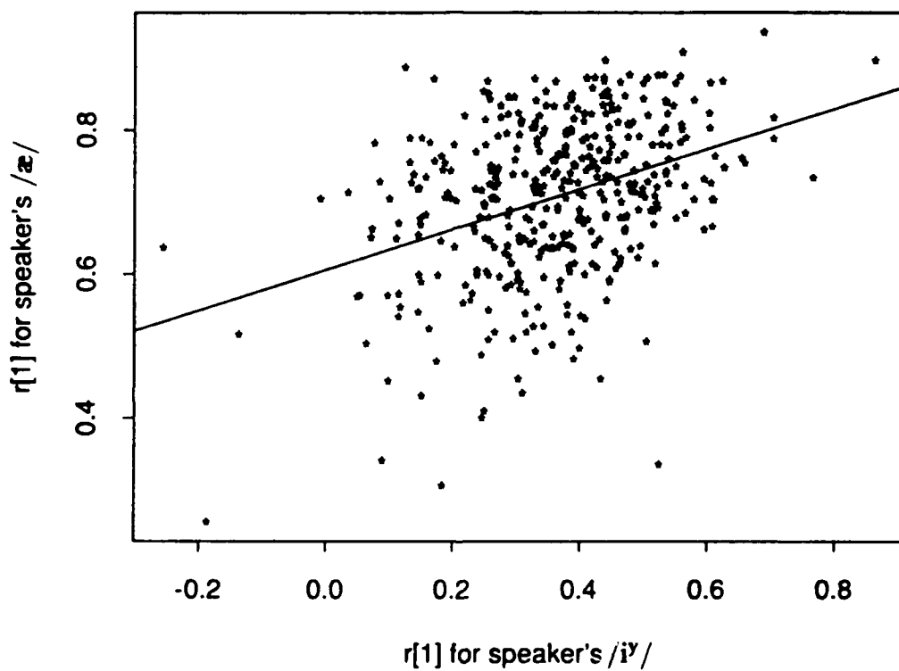
Figure 2.1: Plot of r[1] values for /iʏ/'s and /æ/'s of each speaker. Each point represents a speaker. The x-coordinate of the point is the r[1] for his/her /iʏ/ and the y-coordinate is the r[1] for his/her /æ/.
