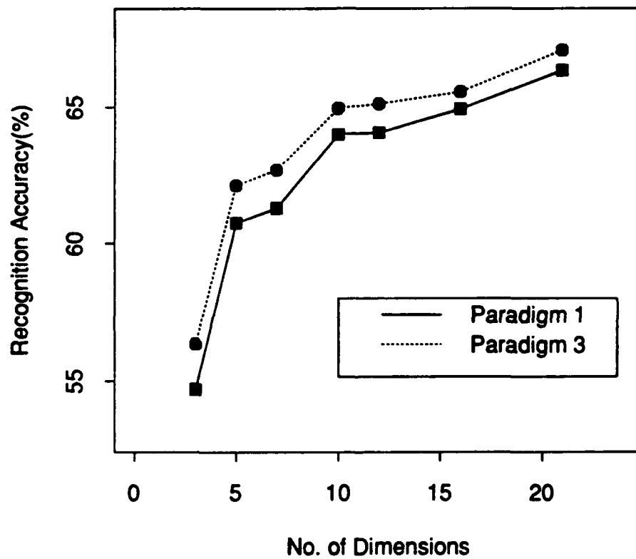
Figure 3.8: Variation of recognition accuracy with number of dimensions. Here the vowel is represented by spectral average of three slices. The data is diagonalized using principal components analysis as described in text.
