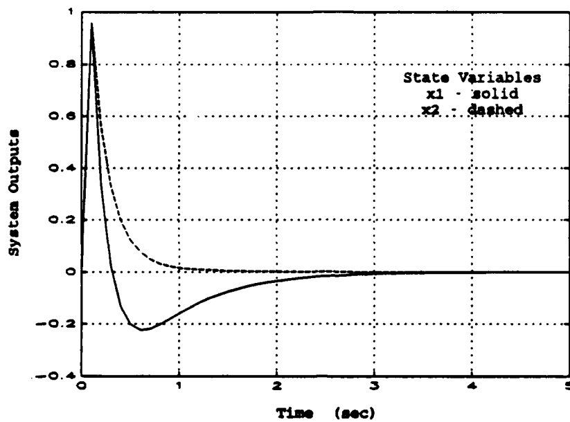
Figure 6. LQR Result for \epsilon = 0.05
