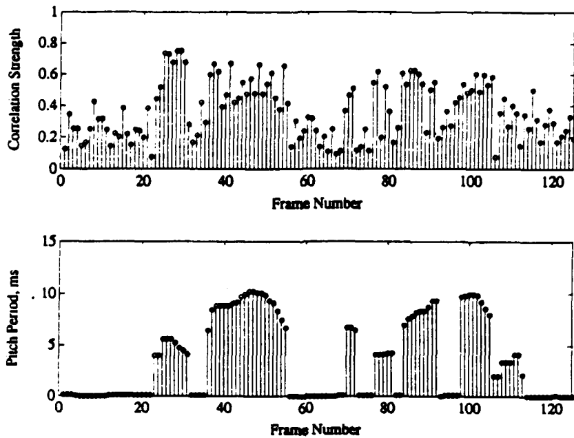
Figure B.1: Correlation strength and pitch period from the standard LPC vocoder. The speech sample is of a male speaker saying "Excuse me madame, would you care to dance?"
