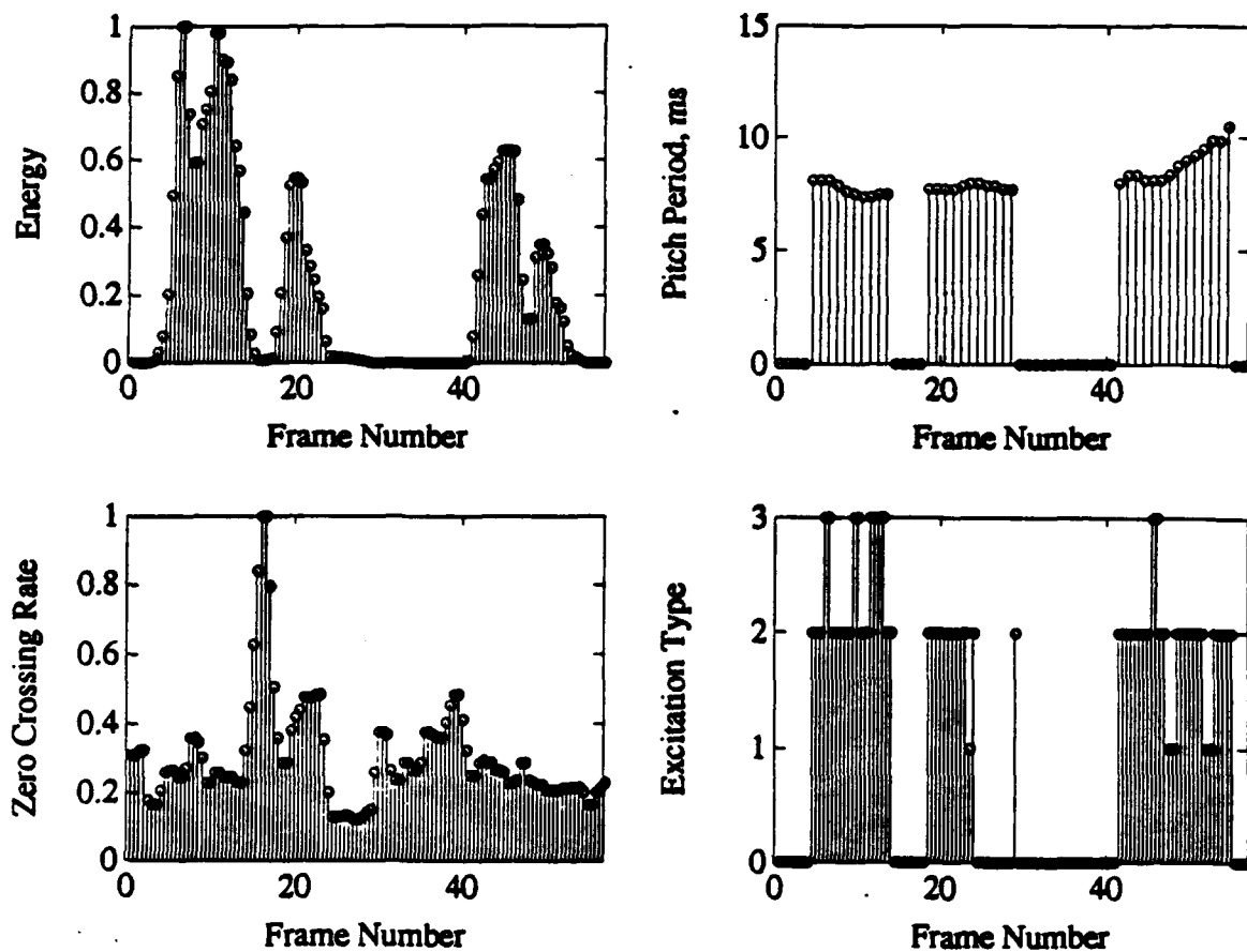
Figure 4.8: Energy, zero crossing rate, pitch period, and excitation type from the four level MME vocoder. The speech sample is of a male speaker saying "Asian cattle." The excitation types are UV for 0, JV1 for 1, JV2 for 2, and VO for 3.
