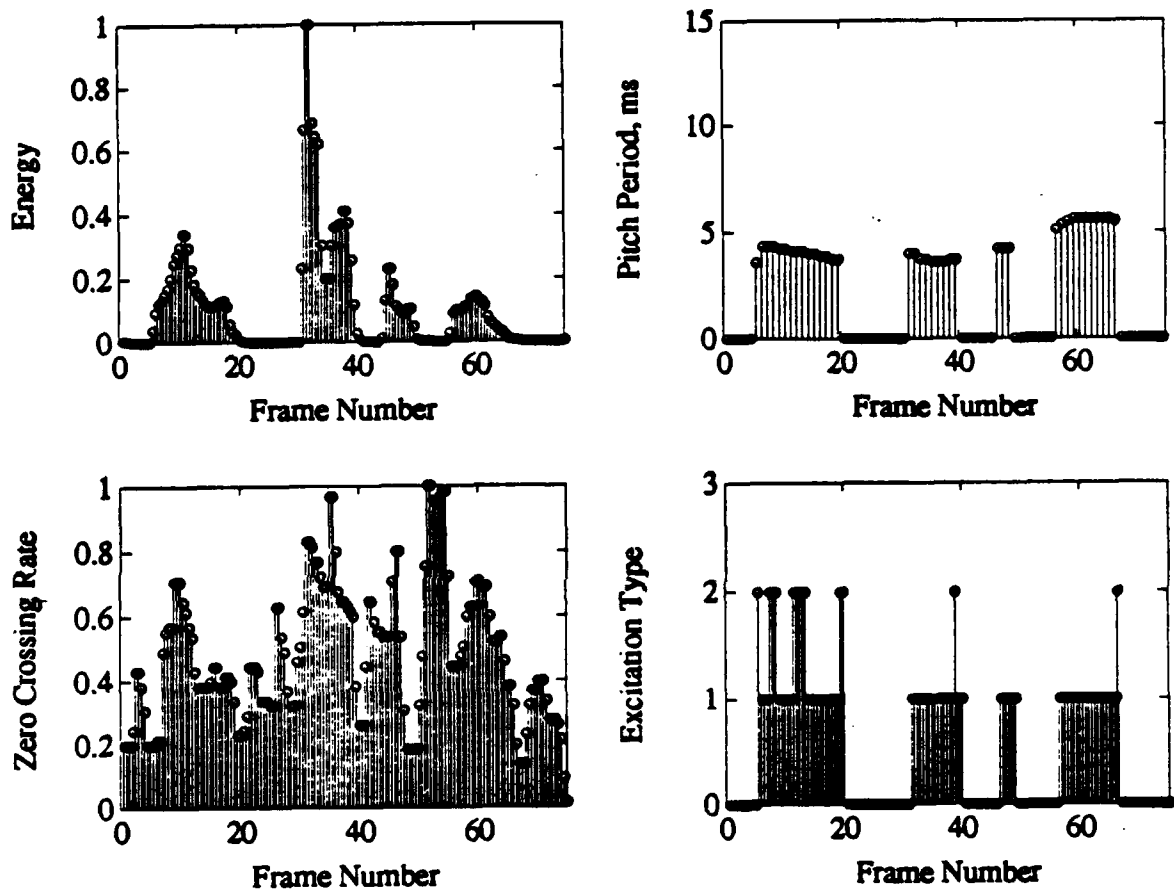
Figure 4.9: Energy, zero crossing rate, pitch period, and excitation type from the four level MME vocoder. The speech sample is of a female speaker saying "No, I don't think so." The excitation types are UV for 0, JV1 for 1, JV2 for 2, and VO for 3.
