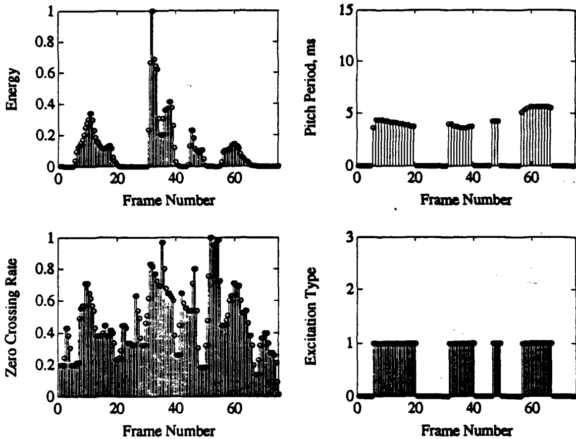
Figure 4.7: Energy, zero crossing rate, pitch period, and excitation type from the MME vocoder. The speech sample is of a female speaker saying "No, I don't think so." The excitation types are UV for 0, JV for 1, and VO for 2.
