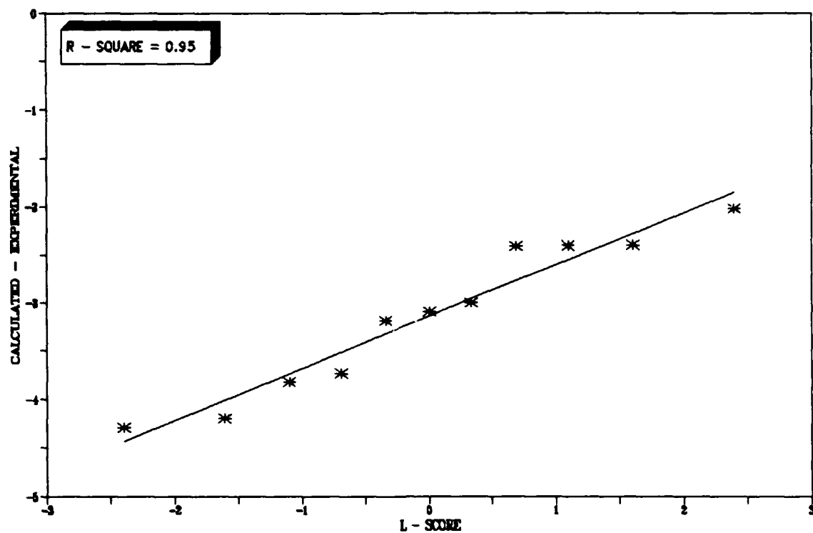
Figure 26. Test for Normal Distribution, Polarizability, PM3
