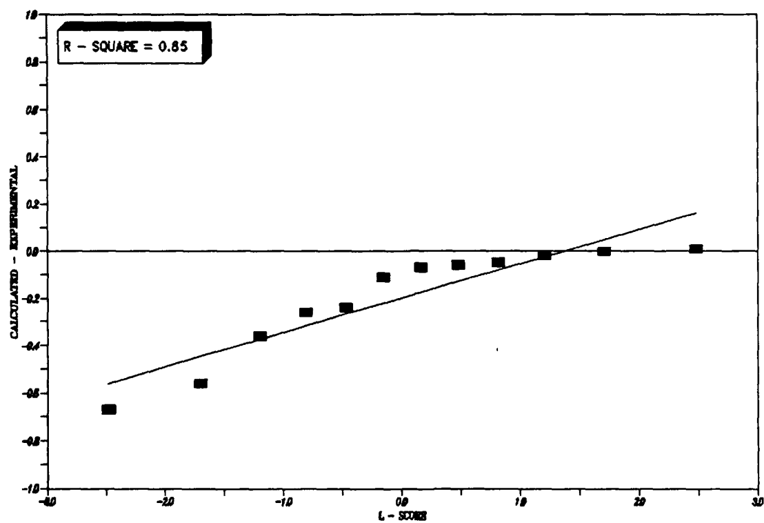
Figure 20. Test for Normal Distribution - Dipole Moment, AM1
