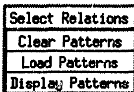
Figure 31: Links Menu
