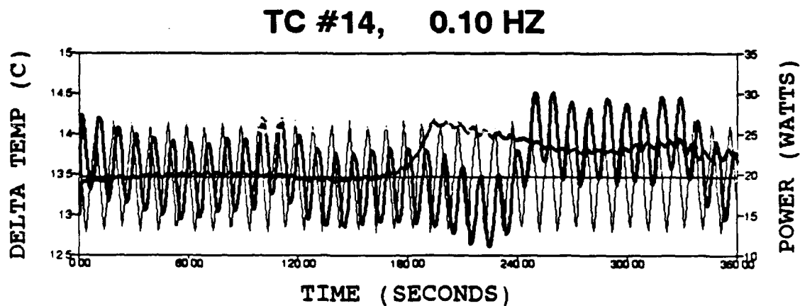
Figure 20. Delta temperature response for steady and cyclic input power with a triangular wave pattern at #14.
