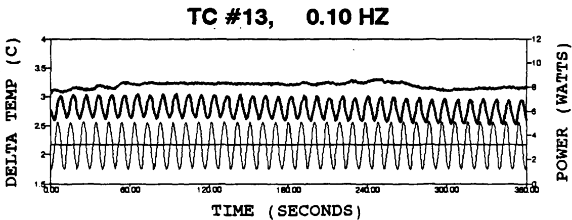
Figure 13. Delta temperature response for steady and cyclic input with sinusoidal wave pattern at #13 for 3.2 W. and R=1.25. Bold=Delta temp response, Fine=Power input.
