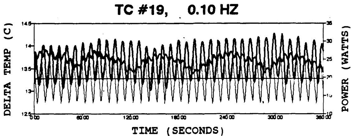
Figure 22. Delta temperature response for steady and cyclic input power with a triangular wave pattern at #19.
