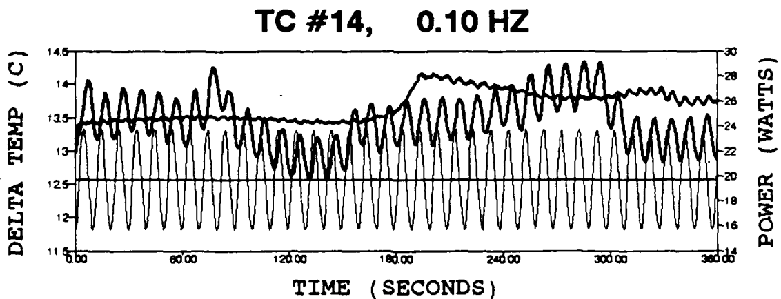
Figure 15. Delta temperature response for steady and cyclic input with sinusoidal wave pattern at #14 for 19.8 W and R=0.404 . Bold=Delta temp response, Fine=Power input
