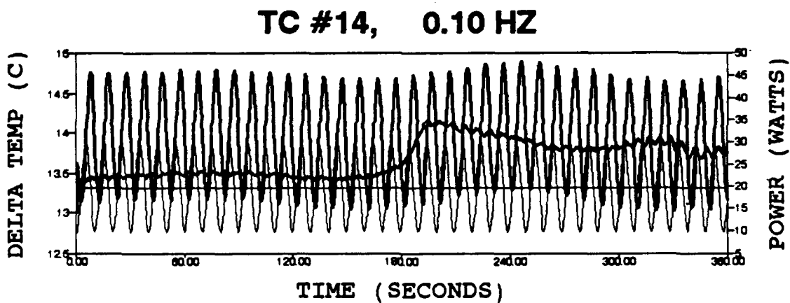
Figure 17. Delta temperature response for steady and cyclic input with sinusoidal wave pattern at #14 for 19.8 W and R=1.010. Bold=Delta temp response, Fine=Power input
