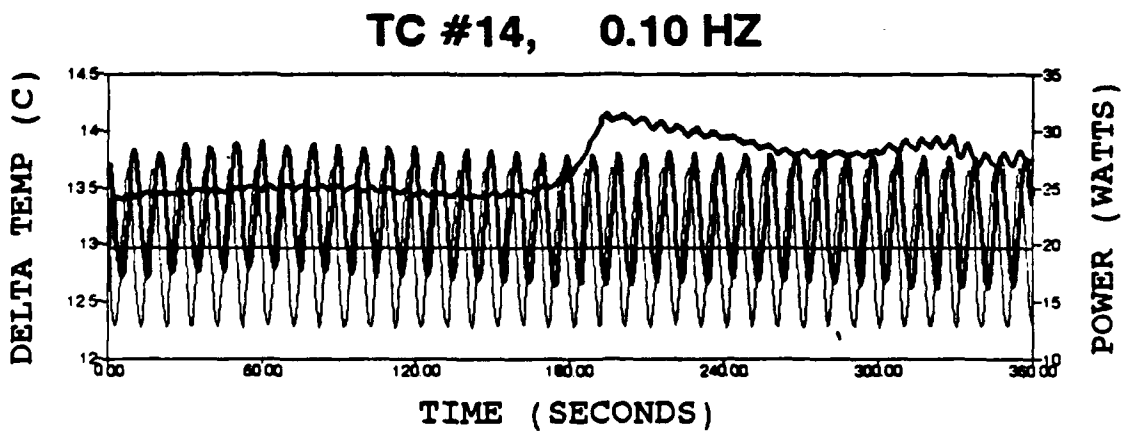
Figure 16. Delta temperature response for steady and cyclic input with sinusoidal wave pattern at #14 for 19.8 W and R=0.707 . Bold=Delta temp response, Fine=Power input
