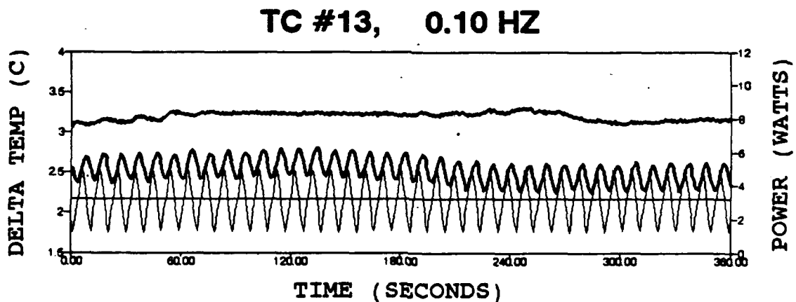
Figure 12. Delta temperature response for steady and cyclic input with triangular wave pattern at #13 for 3.2 W and R=1.25 . Bold=Delta temp response, Fine=Power input.
