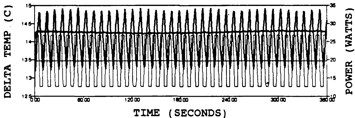
Figure 33. Delta temperature response for steady and cyclic input power with a square wave pattern at #25.
