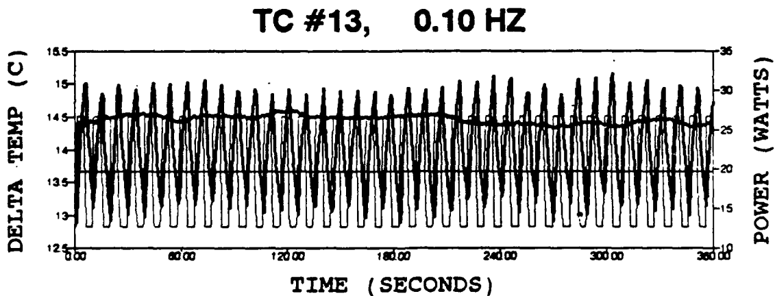
Figure 18. Delta temperature response for steady and cyclic input with square wave pattern at #13 for 19.8 W and R=0.707 . Bold=Delta temp response, Fine=Power input
