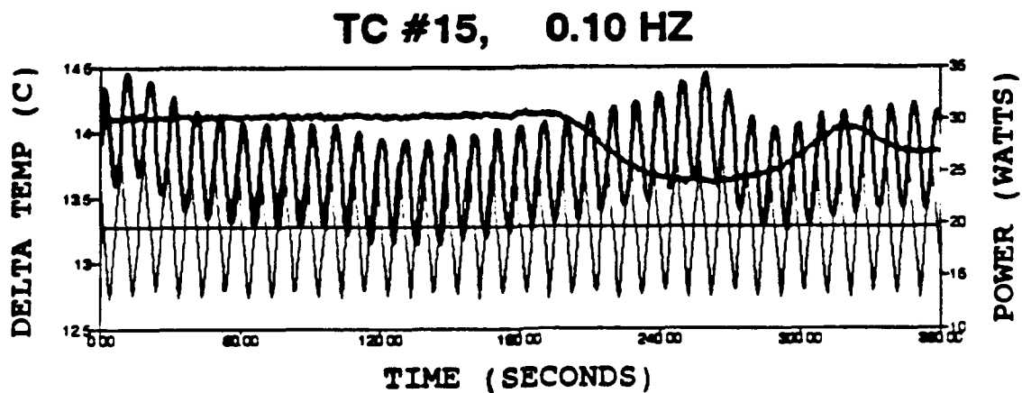
Figure 21. Delta temperature response for steady and cyclic input power with a triangular wave pattern at #15.
