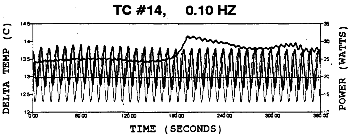
Figure 25. Delta temperature response for steady and cyclic input power with a sinusoidal wave pattern at #14.
