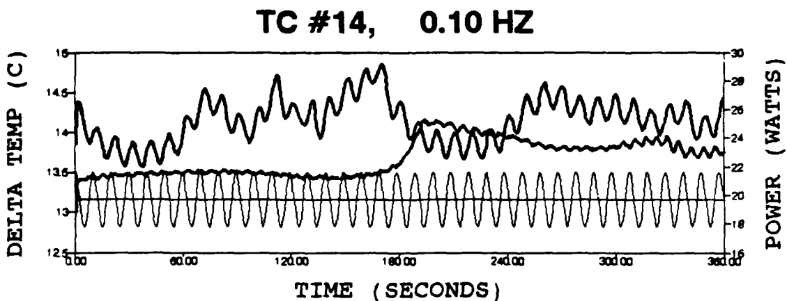
Figure 14. Delta temperature response for steady and cyclic input with sinusoidal wave pattern at #14 for 19.8 W and R=0.202 . Bold=Delta temp response, Fine=Power input.
