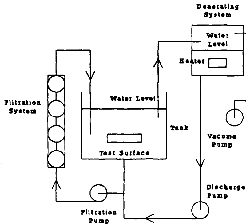
Figure 7. Deaerating/Filtration Assembly
