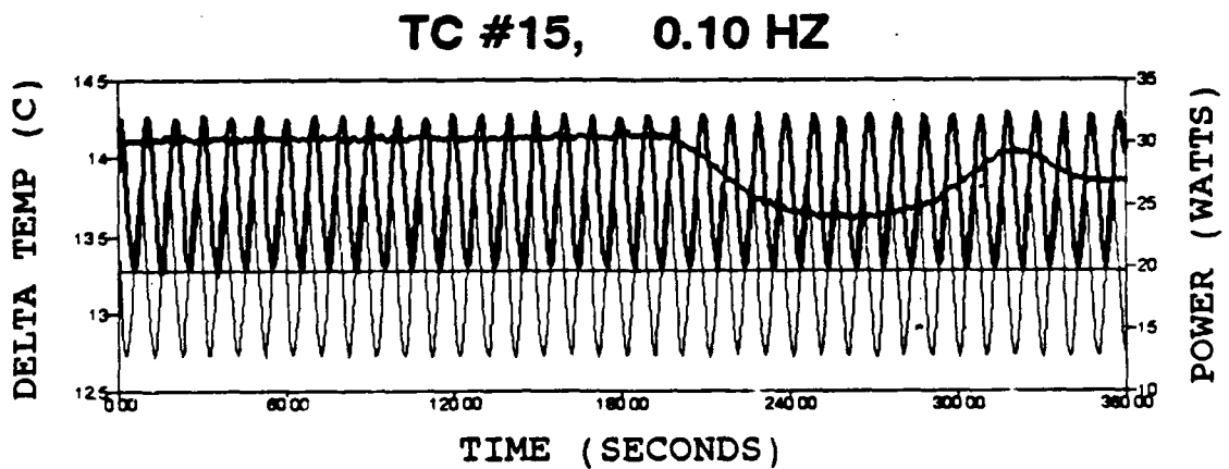
Figure 26. Delta temperature response for steady and cyclic input power with a sinusoidal wave pattern at #15.
