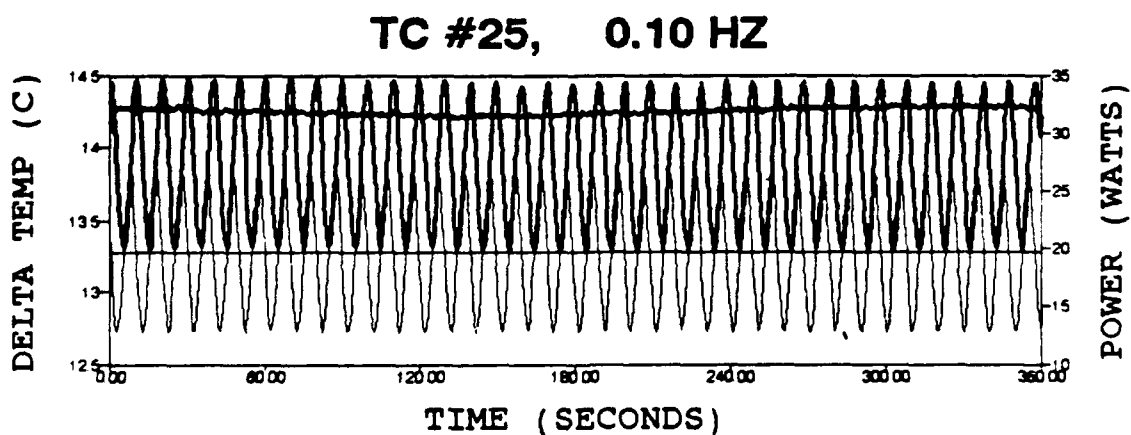
Figure 28. Delta temperature response for steady and cyclic input power with a sinusoidal wave pattern at #25.
