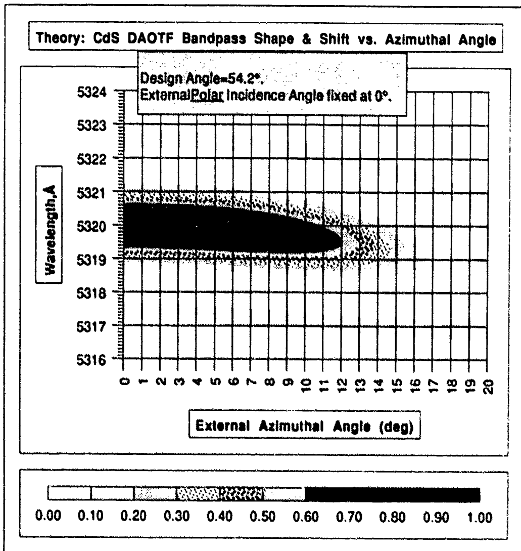
Figure 2-13 Theoretical Bandpass Shape vs. Azimuthal Angle
