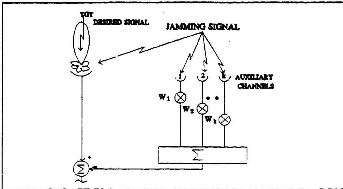
Figure 5.2 A Simplified Block Diagram of Sidelobe Canceler
