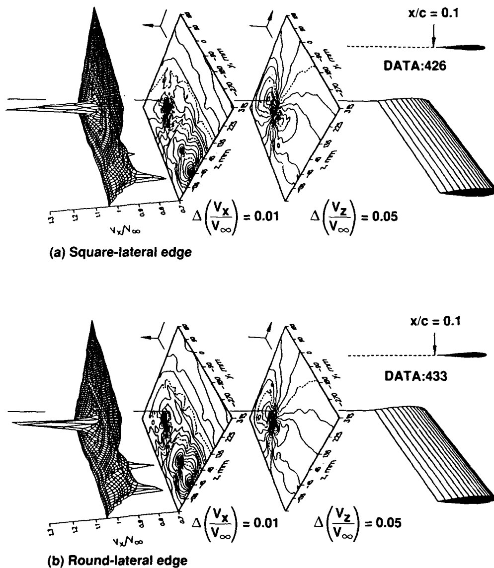
Figure 69. Vertical and streamwise velocity contours around trailing vortex from c = 52 cm wing ( AR = 6.6 ) at Re = 2.0 \times 10^6 and \alpha = 12^\circ for square- and round-lateral edges.
