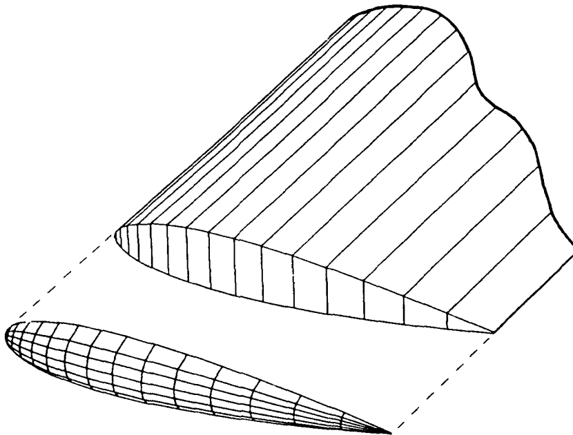
Figure 1. NACA 0015 wing with square tip, and end cap for forming round tip.
