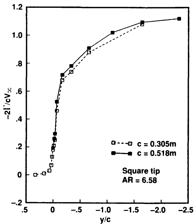
Figure 38. Comparison of circulation along wing span at \alpha = 12^\circ and Re = 1.5 \times 10^6 .
