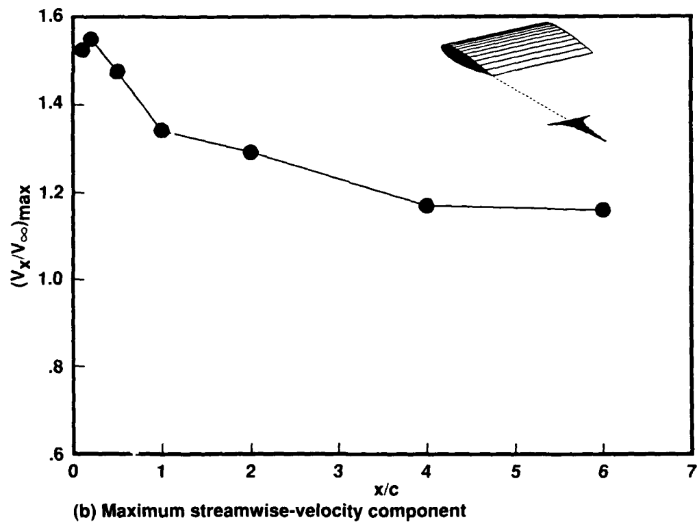
Figure 40. Downstream change in maximum vertical and streamwise velocities within trailing vortex from basic wing with c = 52 cm at Re = 1.5 \times 10^6 and \alpha = 12^\circ .
