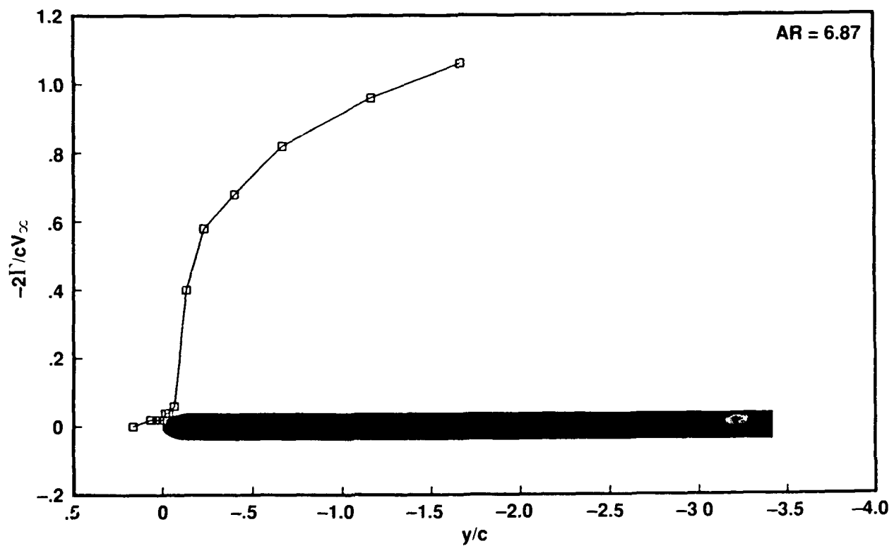
Figure 37. Circulation along wing span at \alpha = 12^\circ and Re = 1.5 \times 10^6 .
