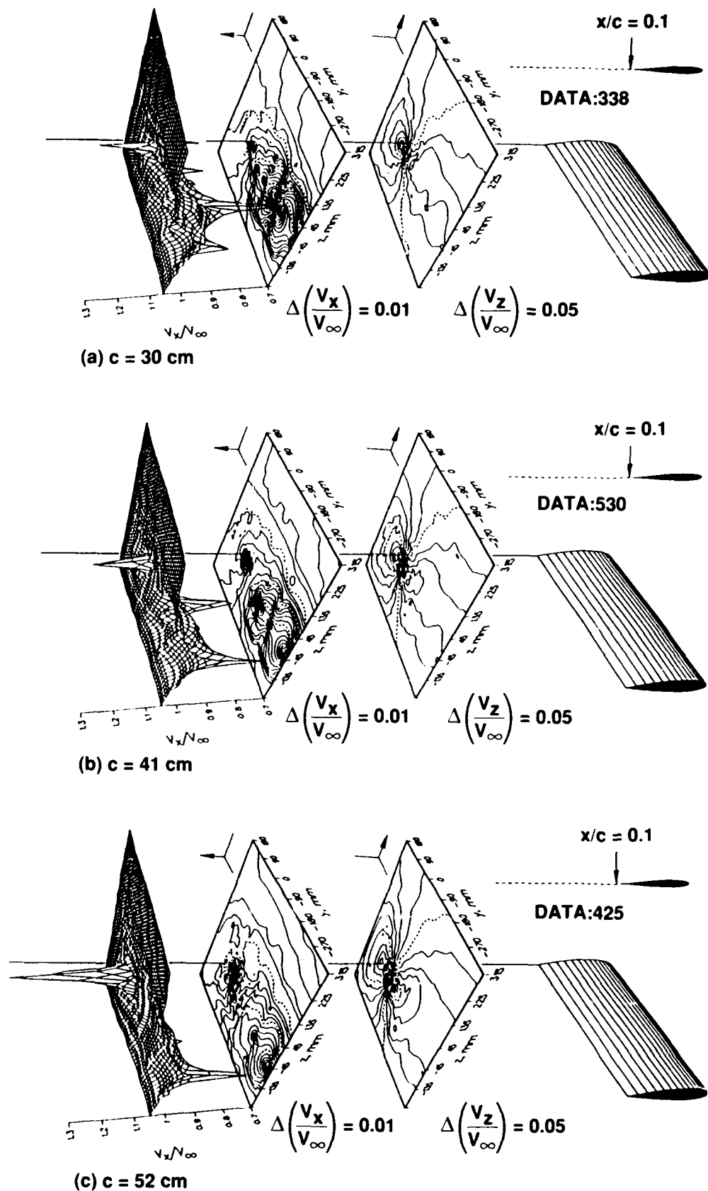
Figure 46. Vertical and streamwise velocity contours around trailing vortex from basic wing at x/c = 0.1 with Re = 1.5 \times 10^6 and \alpha = 12^\circ for different chord lengths while maintaining C_l V_\infty = \text{constant} .
