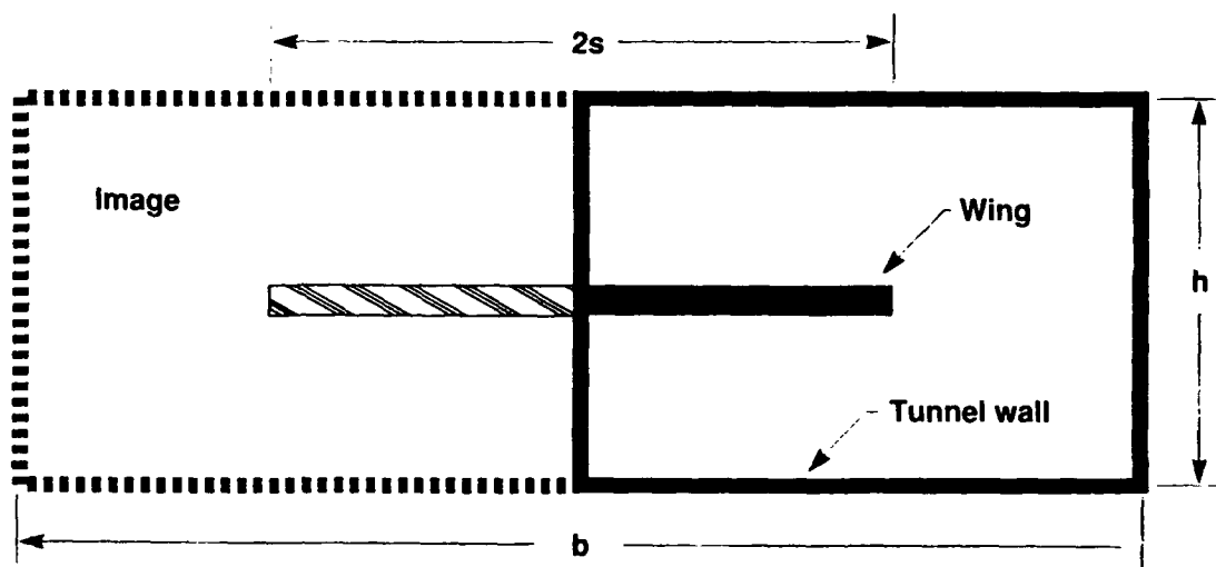
Figure 78. Assumed interference geometry with side-wall reflection.
