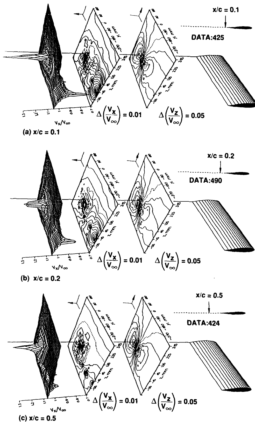
Figure 42. Vertical and streamwise velocity contours around trailing vortex from basic wing with c = 52 cm at Re = 1.5 \times 10^6 and \alpha = 12^\circ measured at different downstream stations.
