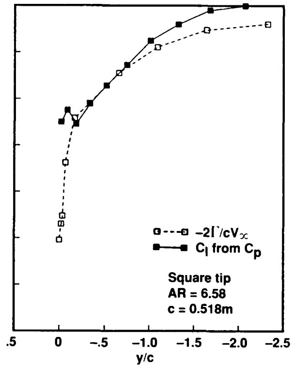
Figure 38. Comparison of circulation along wing span at \alpha = 12^\circ and Re = 1.5 \times 10^6 .
