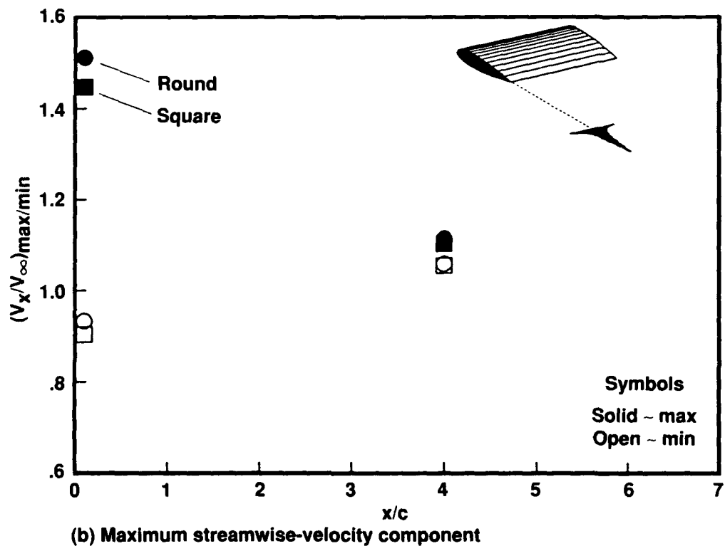
Figure 67. Maximum vertical and streamwise velocities within trailing vortex from wing ( AR = 6.6 ) at \alpha = 12^\circ for square- and round-lateral edges. Values at x/c = 0.1 for c = 52 cm wing with Re = 2.0 \times 10^6 and those at x/c = 4 for c = 30 cm wing with Re = 1.5 \times 10^6 .
