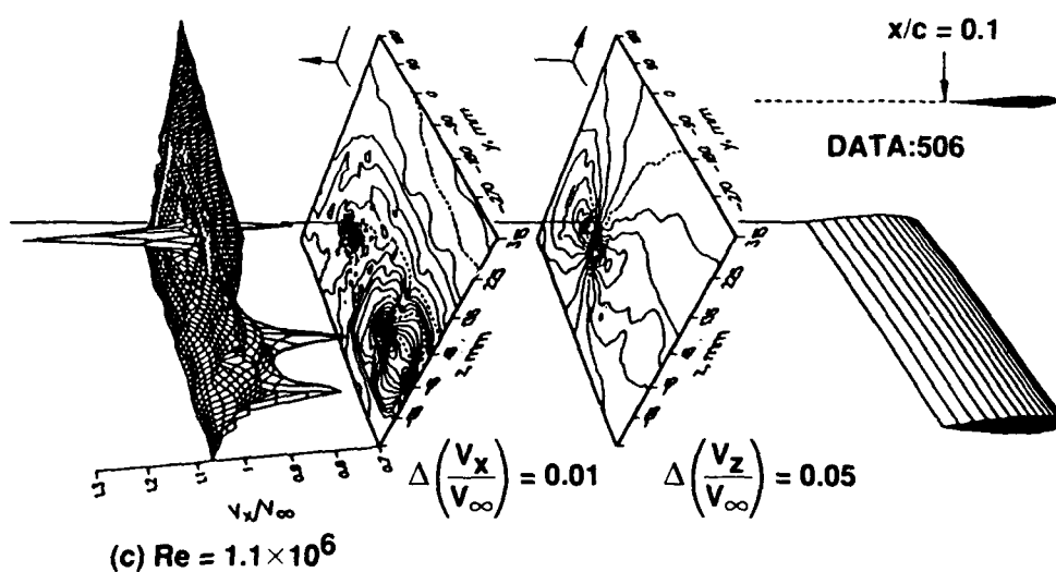
Figure 50. Vertical and streamwise velocity contours around trailing vortex from basic wing with c = 52 cm at x/c = 0.1 for different Reynolds numbers while maintaining C_l V_\infty = \text{constant} .
