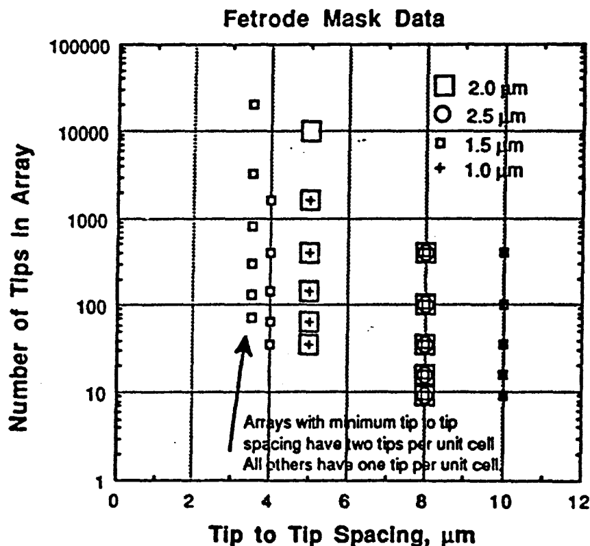
Fig. 1 - Graphic description of the size and spacing of emitter tip arrays on mask set #1.
