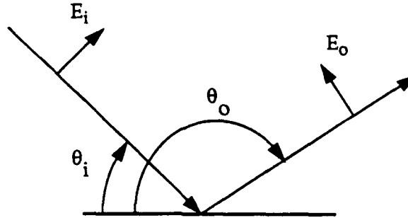
Figure I.1 Incident and scattered angle geometry.
