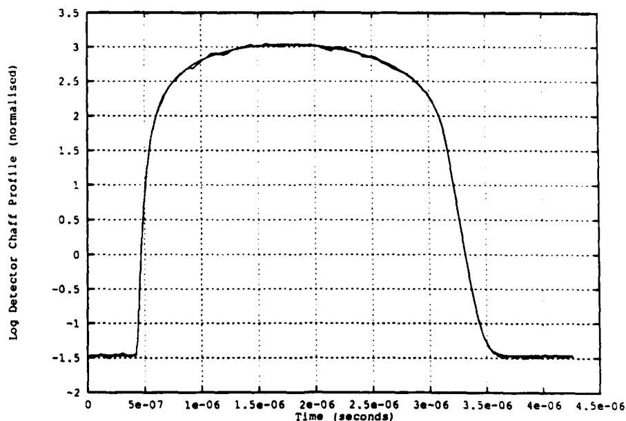
Figure 7 The average over 1000 samples for the log detector of the received signal, using the 0.1 \mu s radar. The maximum ensemble average RCS obtained is 400 \text{m}^2 .
