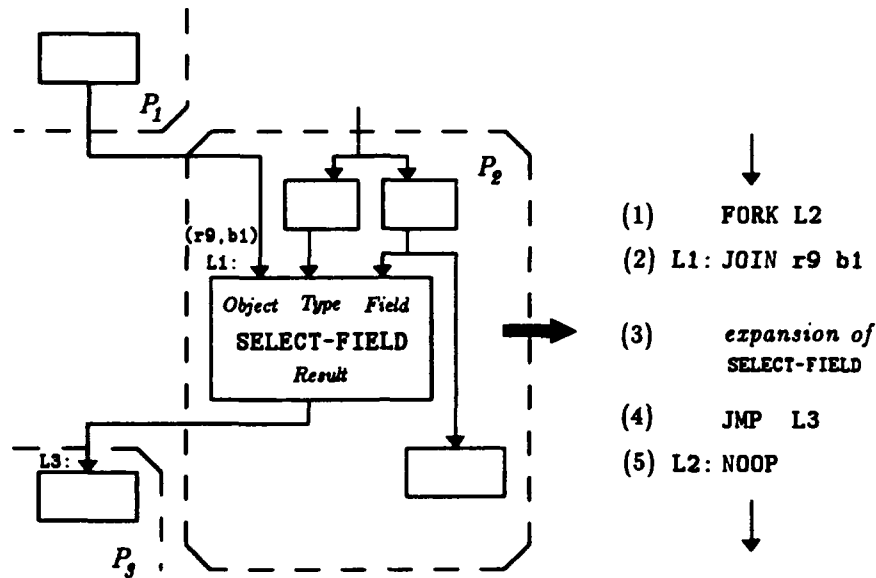
Figure 4.27: Explicit synchronization and control transfers.
