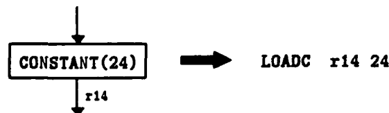
Figure 4.28: Expansion of CONSTANT(24) .
