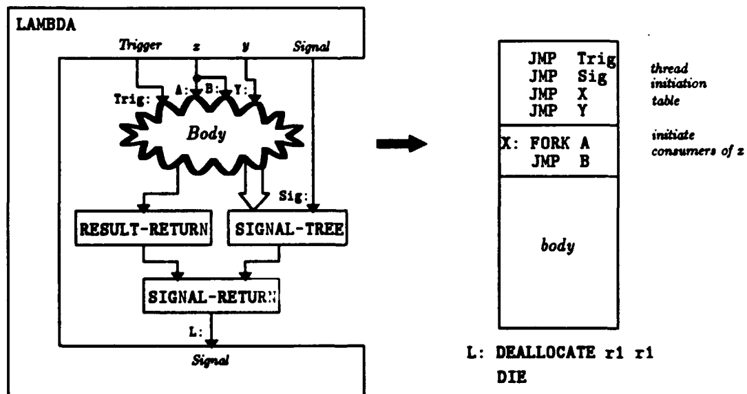
Figure 4.32: Organization of code in procedure body.
