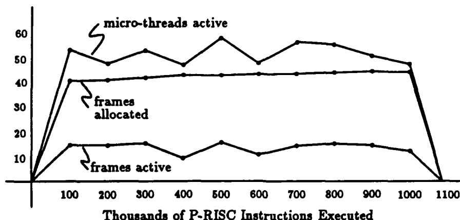
Figure 6.8: Parallelism profile.
