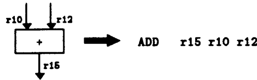
Figure 4.29: Expansion of +.
