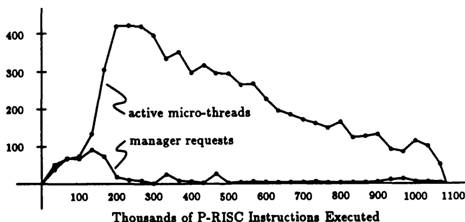
Figure 6.7: Parallelism profile of forward traverse operation.
