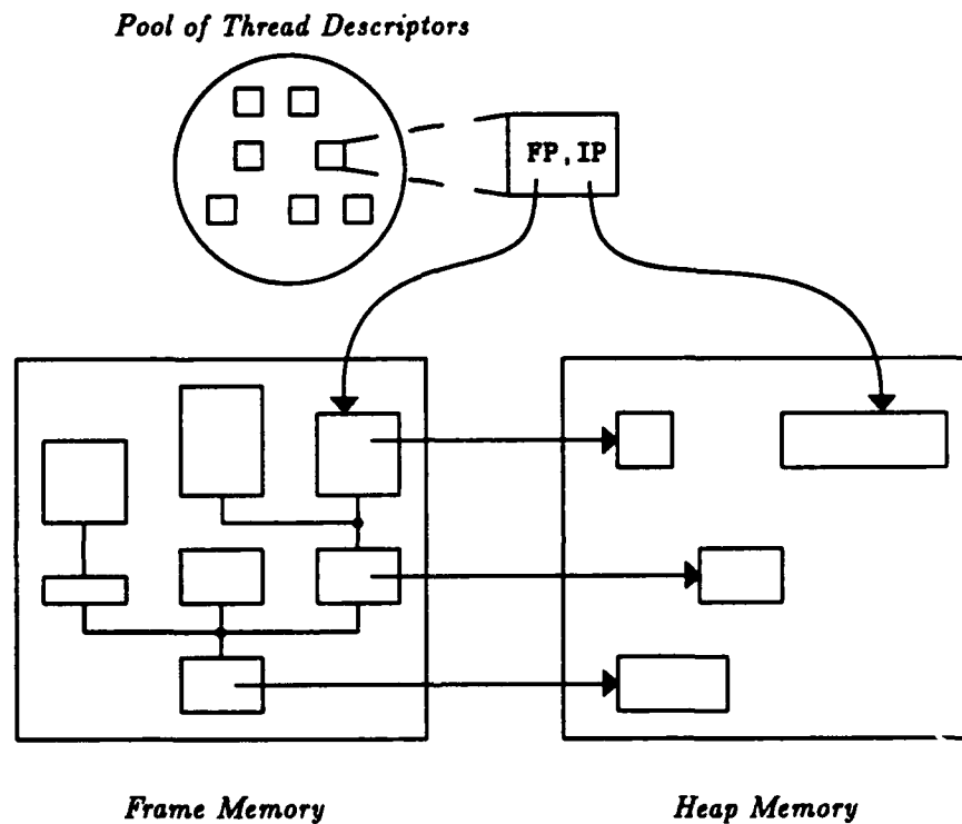
Figure 4.18: Organization of P-RISC abstract machine.
