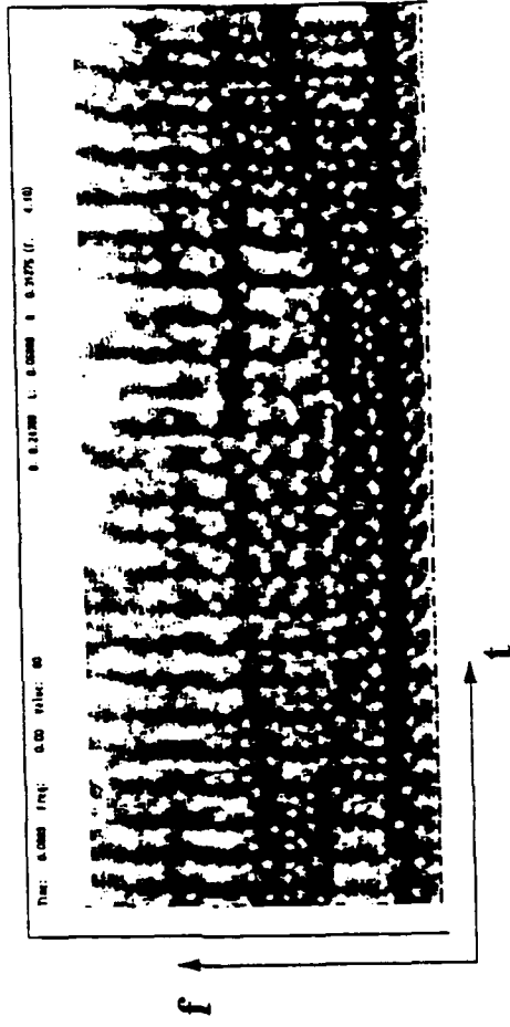
Wideband Spectrogram (short h(t) ): "joy"
