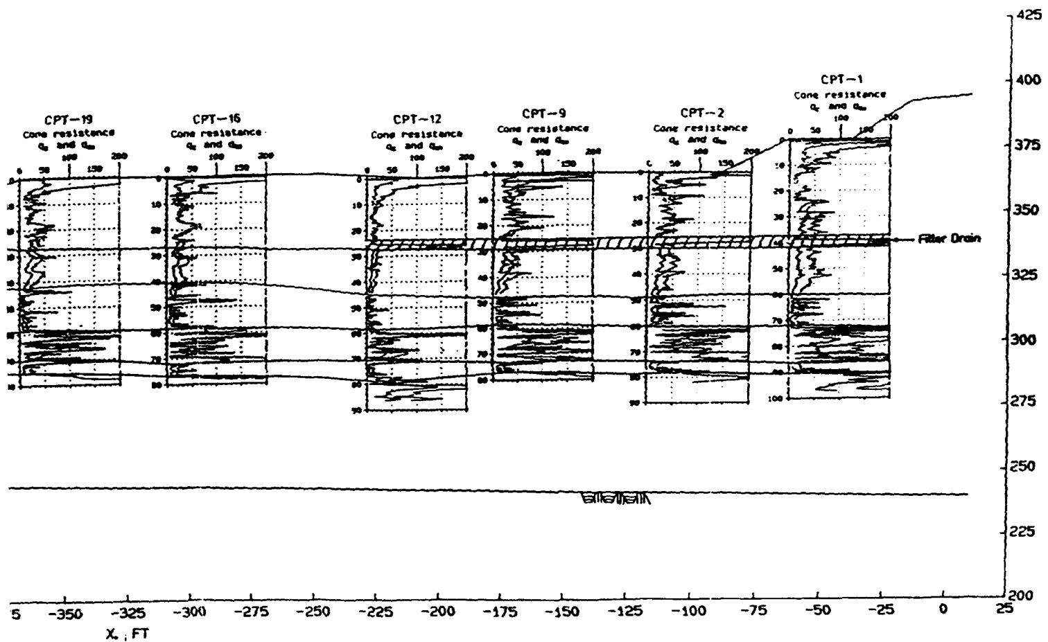
CPT cone resistance along section D'-D' perpendicular to the axis of the dam).
