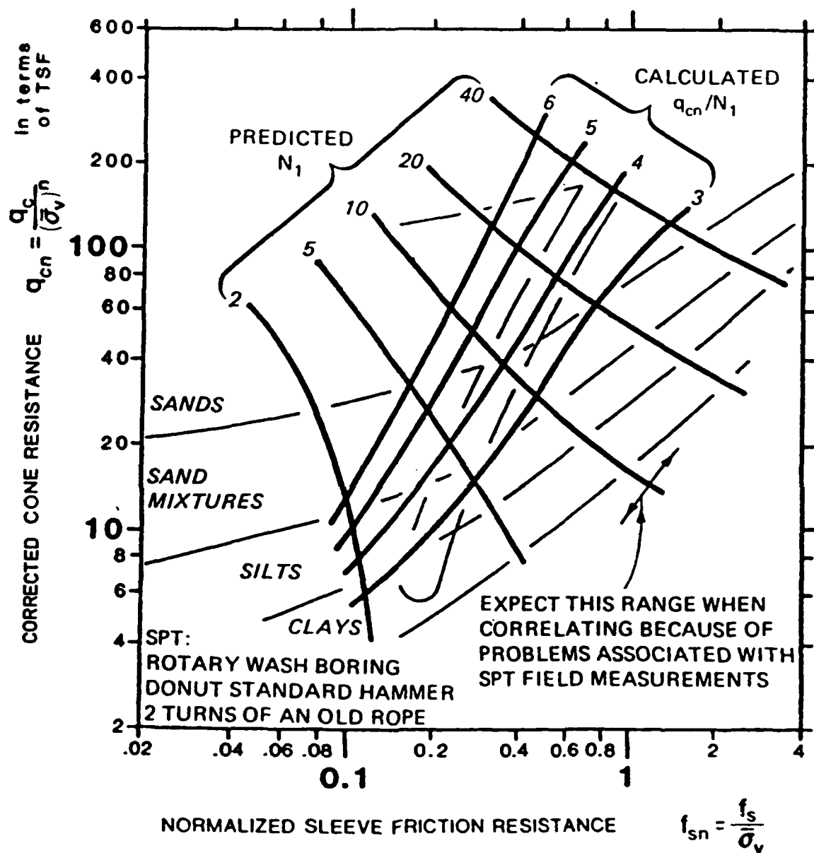
Figure 82. Chart used for CPT prediction of (N_1)_{60} .
