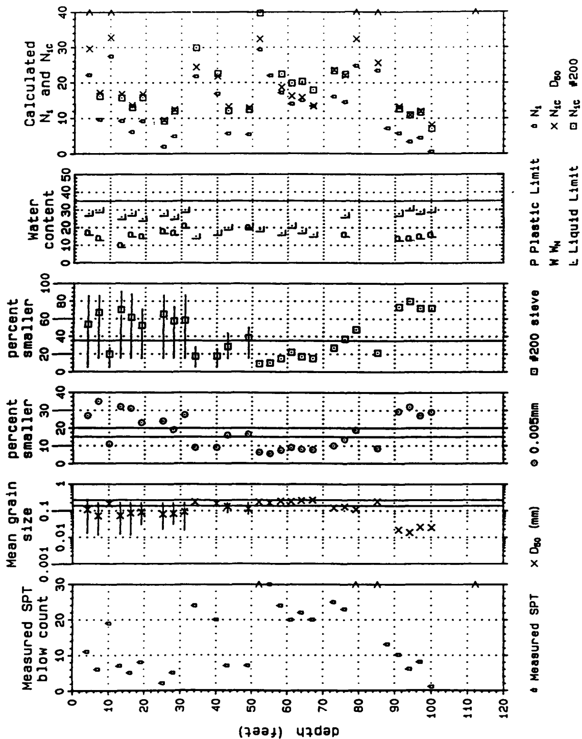
BEQ-06 Barkley dam SPT Liquefaction Analysis
