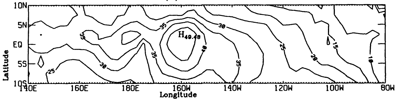
MIXED LAYER DEPTH (m) JANUARY 1986
