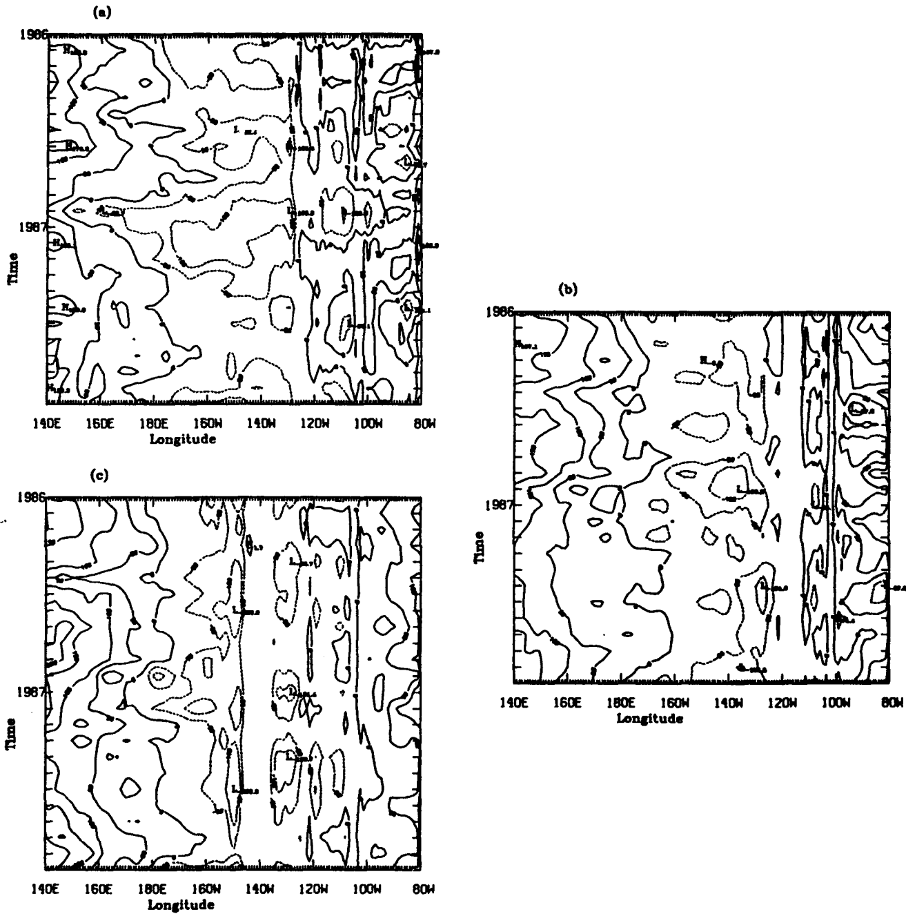
Figure 8. Time evolution of net surface heat flux ( Q_0 ) for latitudes (a) 5N, (b) 0, and (c) 5S across the equatorial Pacific. The value of Q_0 is defined as positive (solid) downwards, and negative (dashed) upwards.
