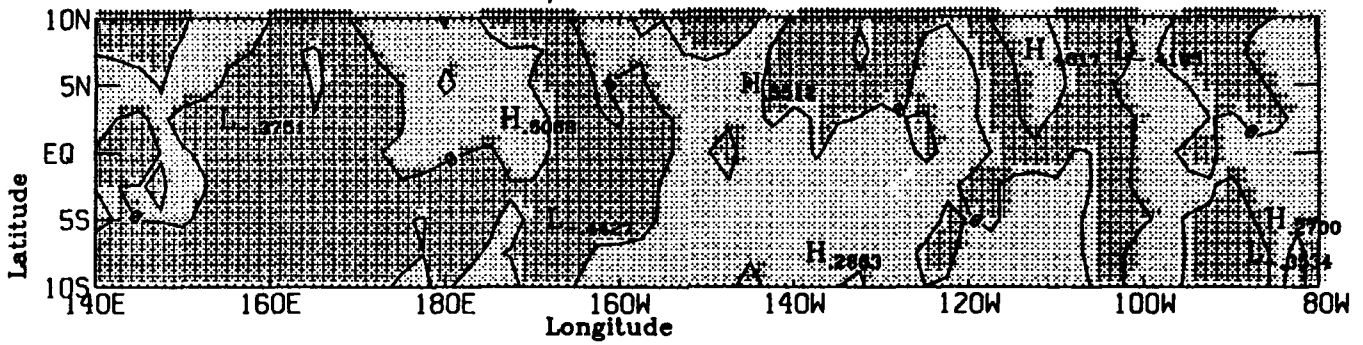
CORRELATION OF dT_s/dt and h AUGUST 1986
