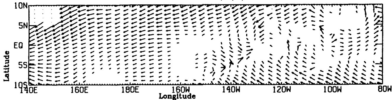
WATER SURFACE FRICTION VELOCITY (CM/S) APRIL 1988
