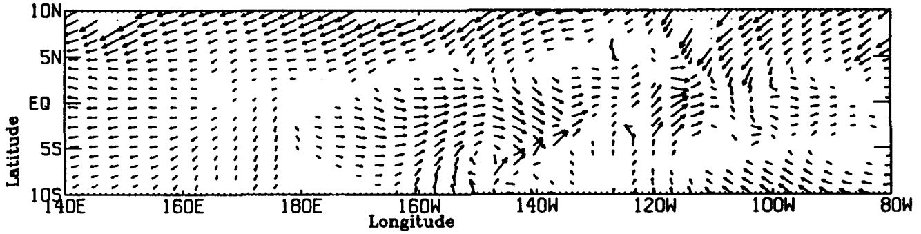
WATER SURFACE FRICTION VELOCITY (CM/S) NOVEMBER 1988
