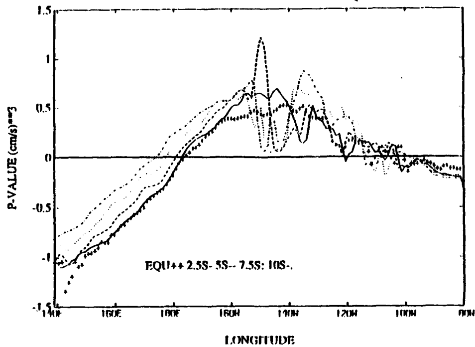
Figure 12. Average P-values for latitudes (a) 10N through 0, and (b) 0 through 10S across the equatorial Pacific.
