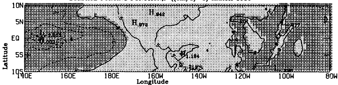
SURFACE FORCING FUNCTION, P ((cm/s)**3) MARCH 1986
