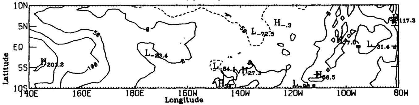
NET SURFACE HEAT FLUX (W/m**2) OCTOBER 1986
