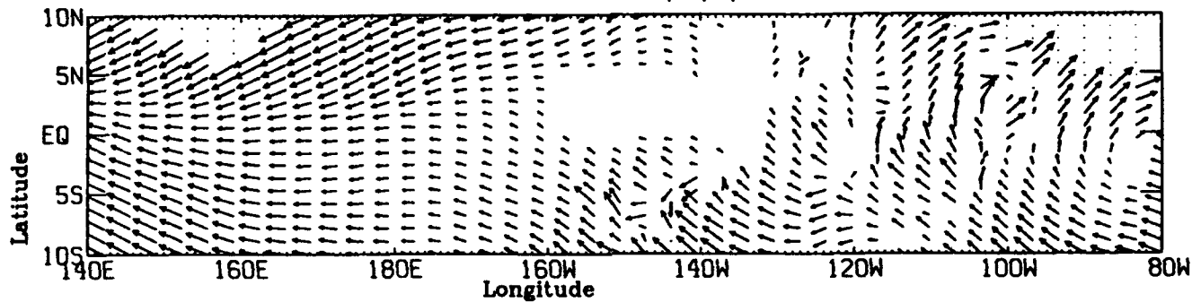
WATER SURFACE FRICTION VELOCITY (CM/S) JUNE 1988
