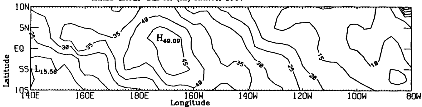
MIXED LAYER DEPTH (m) MARCH 1987
