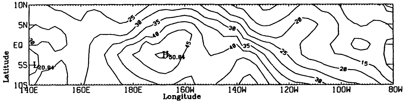
MIXED LAYER DEPTH (m) AUGUST 1986
