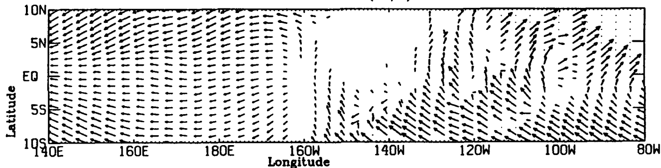
WATER SURFACE FRICTION VELOCITY (CM/S) MAY 1988
