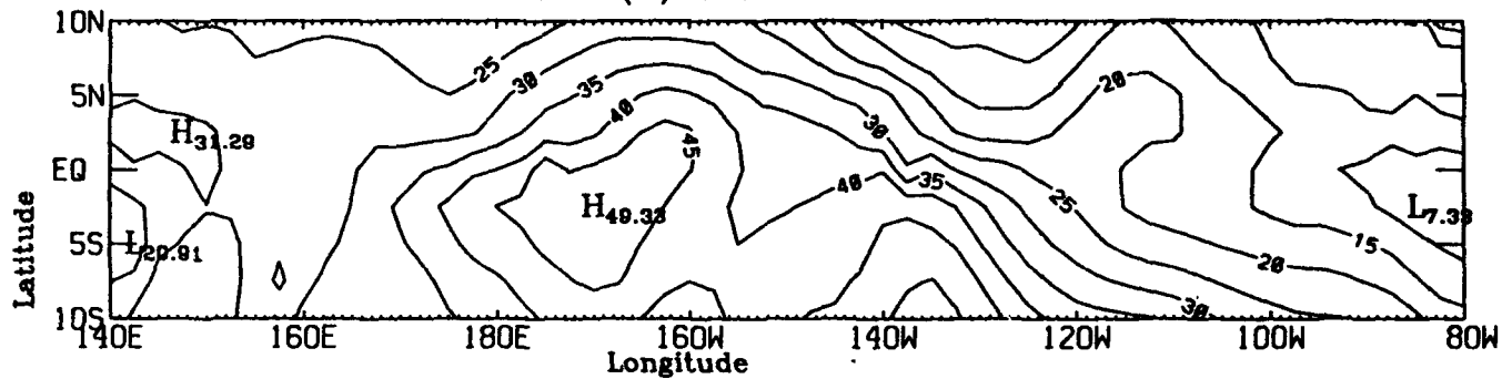
MIXED LAYER DEPTH (m) SEPTEMBER 1987
